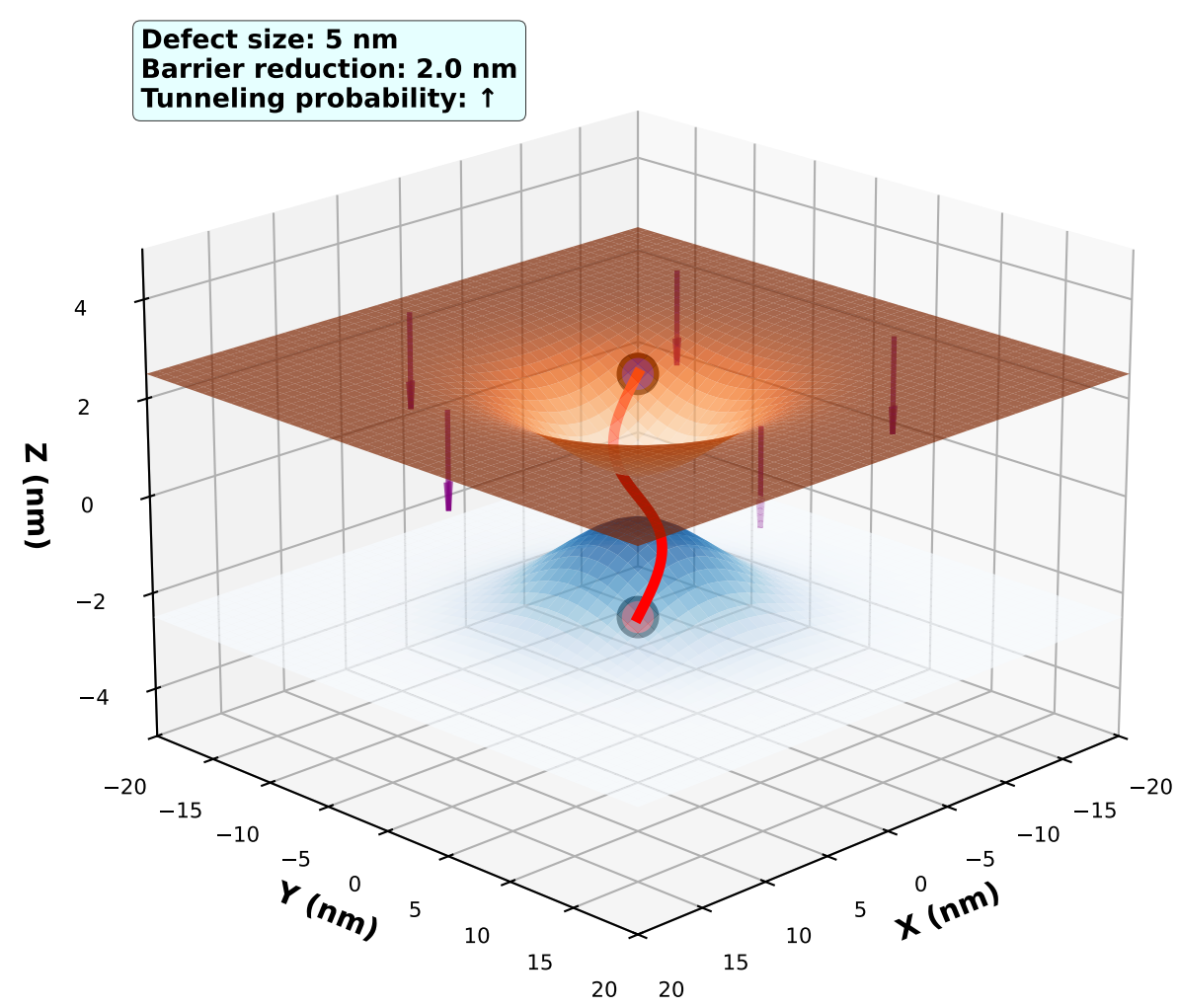
(C) Membrane Defect: Quantum Tunneling Pathway
