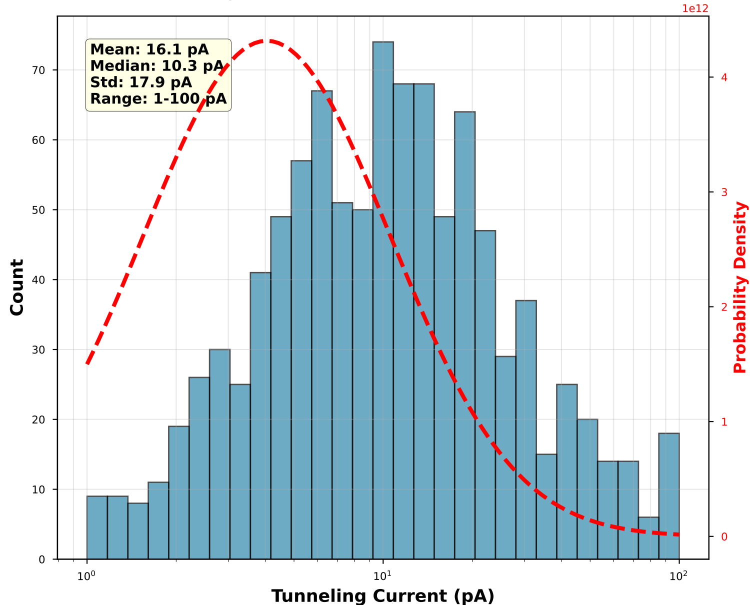
(C) Membrane Defect: Quantum Tunneling Pathway
