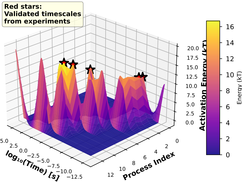
(C) Energy Landscape: Multi-Scale Dynamics
