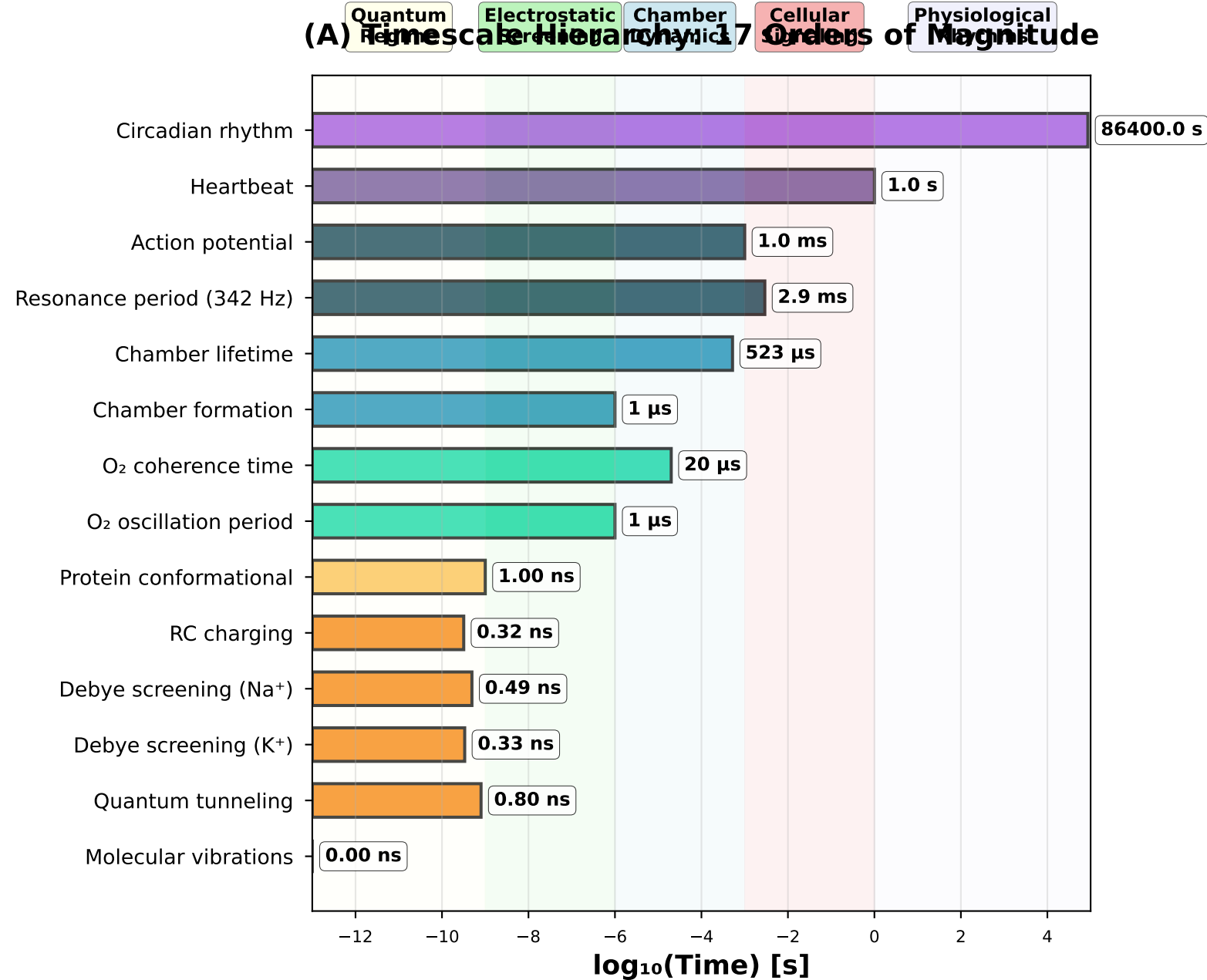
Figure 8: Integrated Timescale Hierarchy & Physiological Coherence
