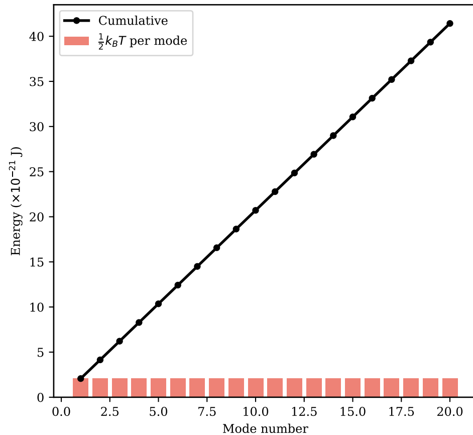
Equipartition
