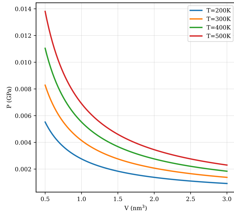
Isotherms
