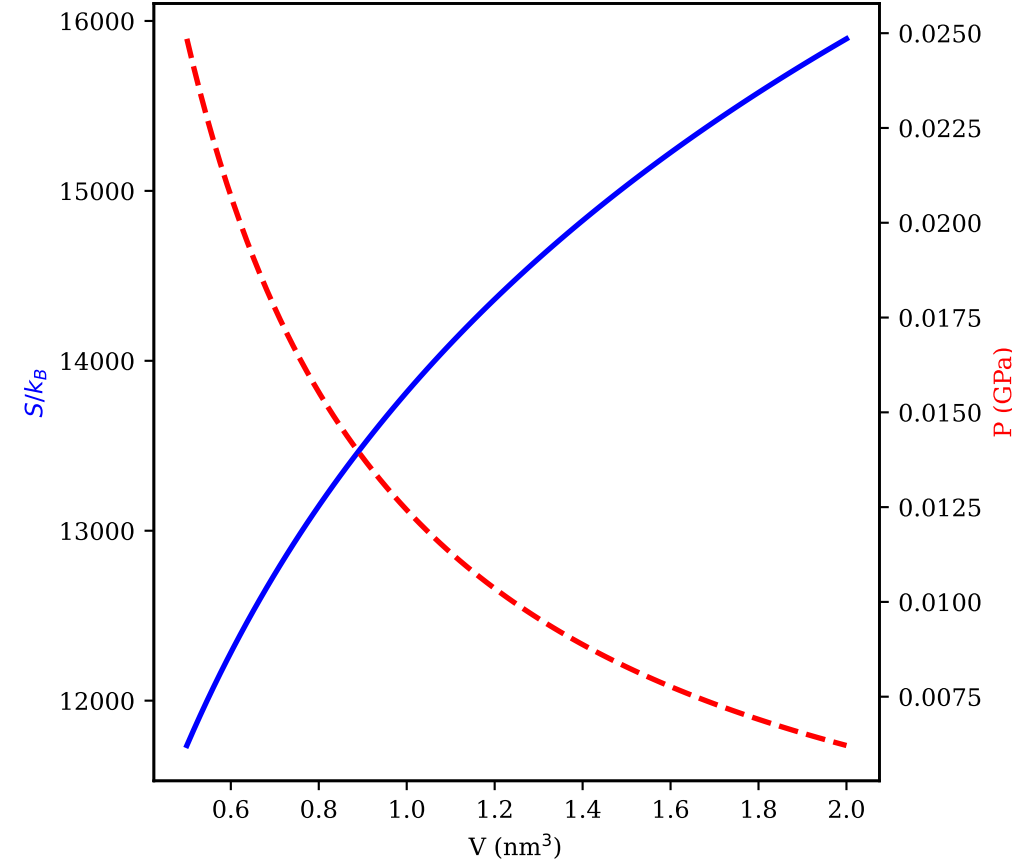
P = T(\partial S / \partial V)
