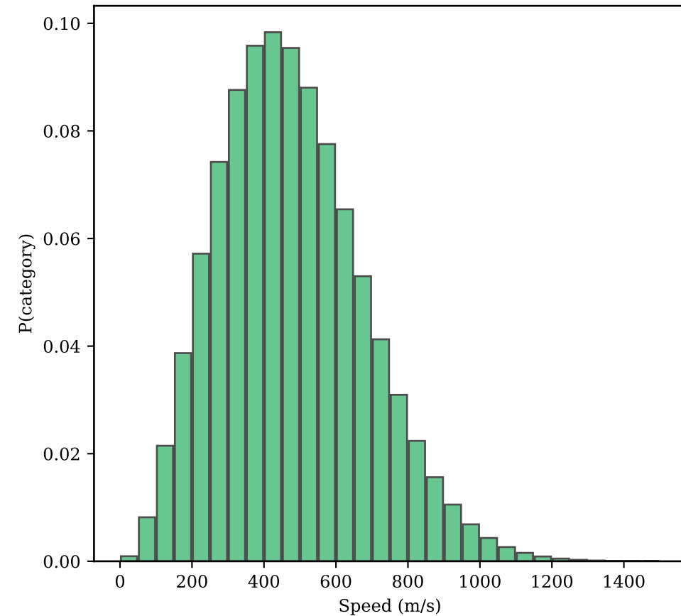
Categorical Discretization
