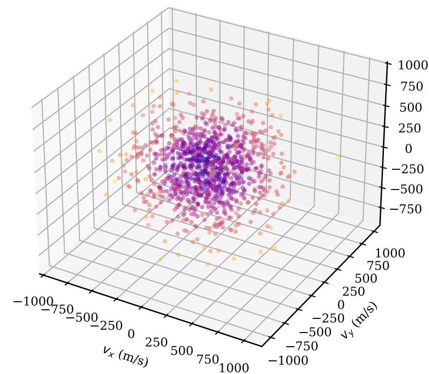
3D Velocity Distribution
