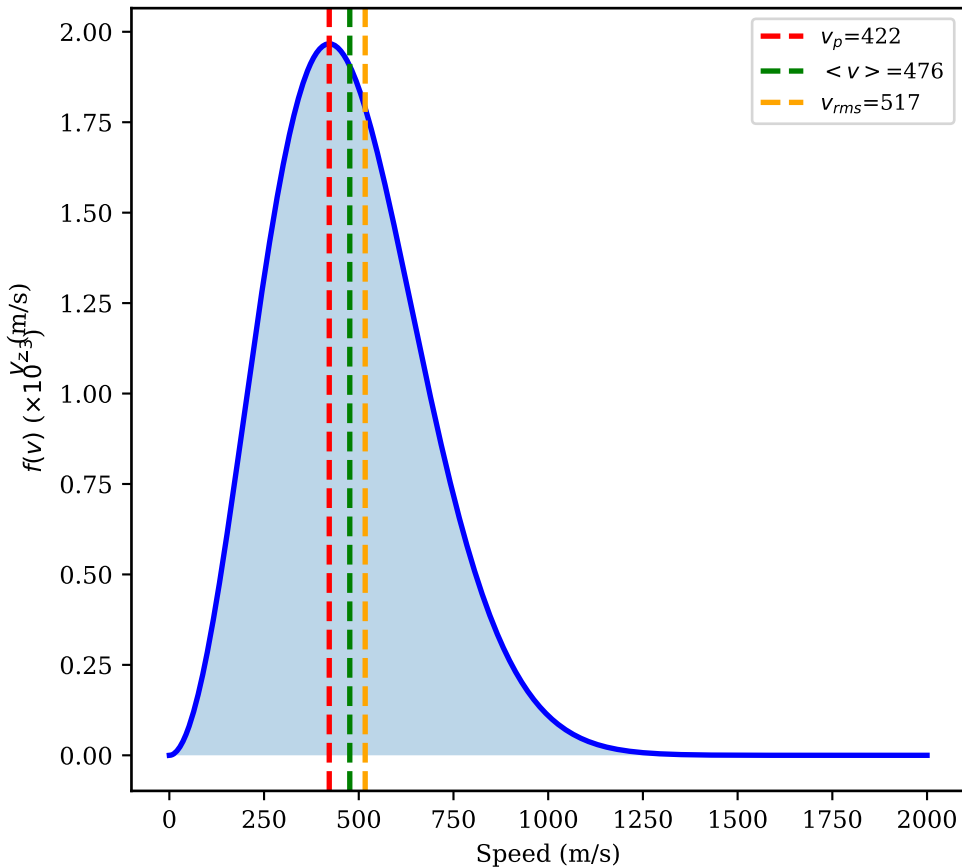
Maxwell-Boltzmann
