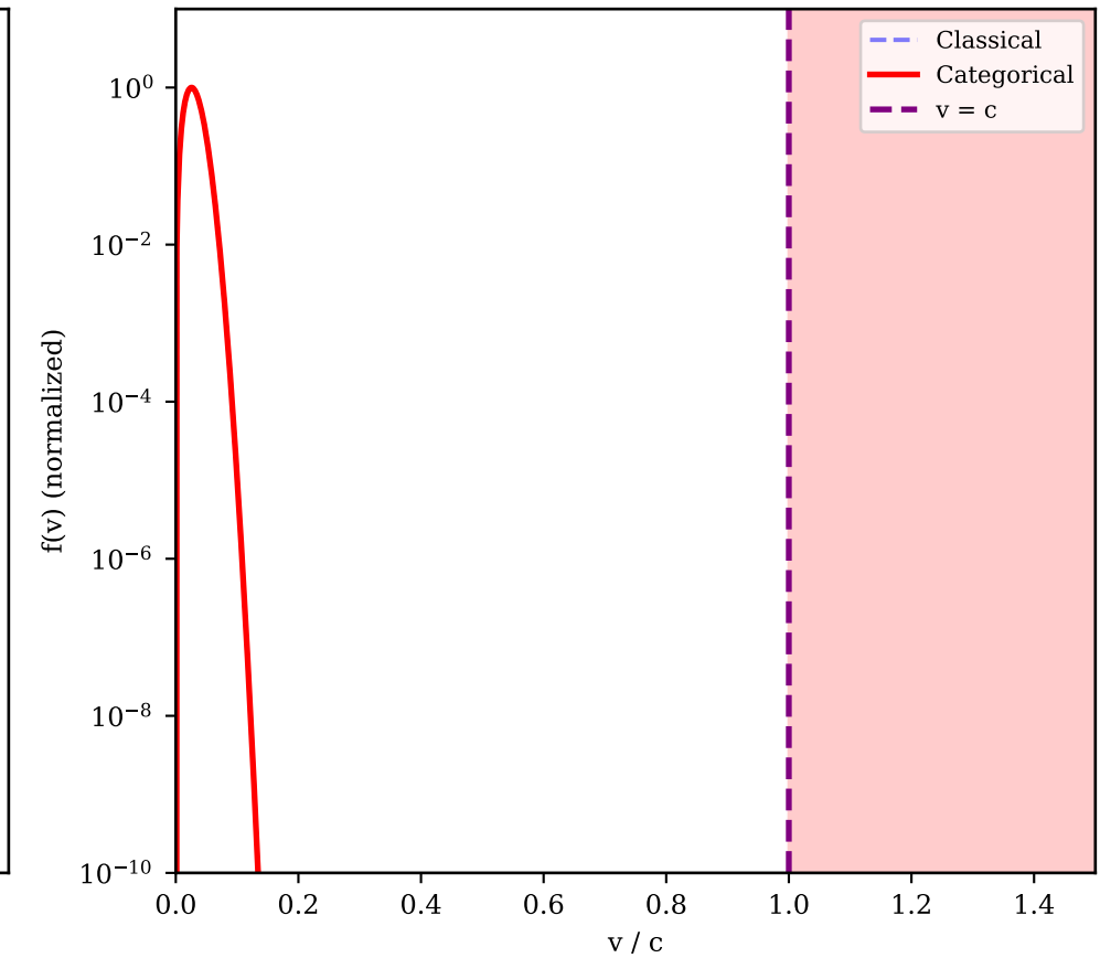
Cutoff at v = c ( T = 10^{11} K)
