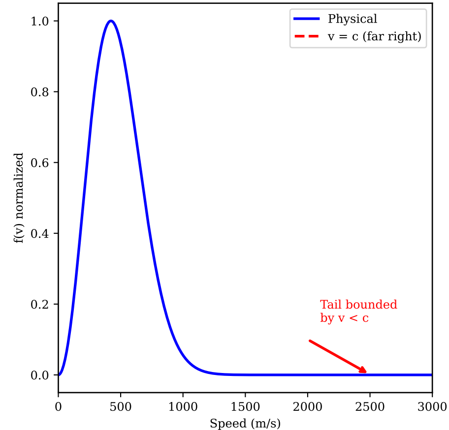
Bounded Distribution
