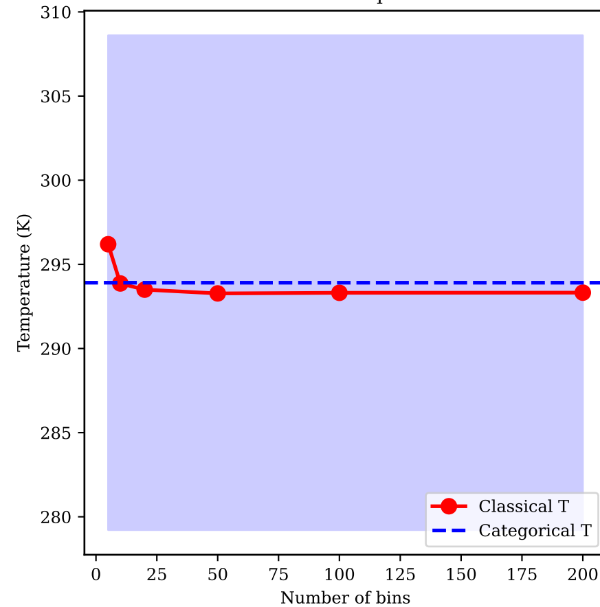
Resolution Independence
