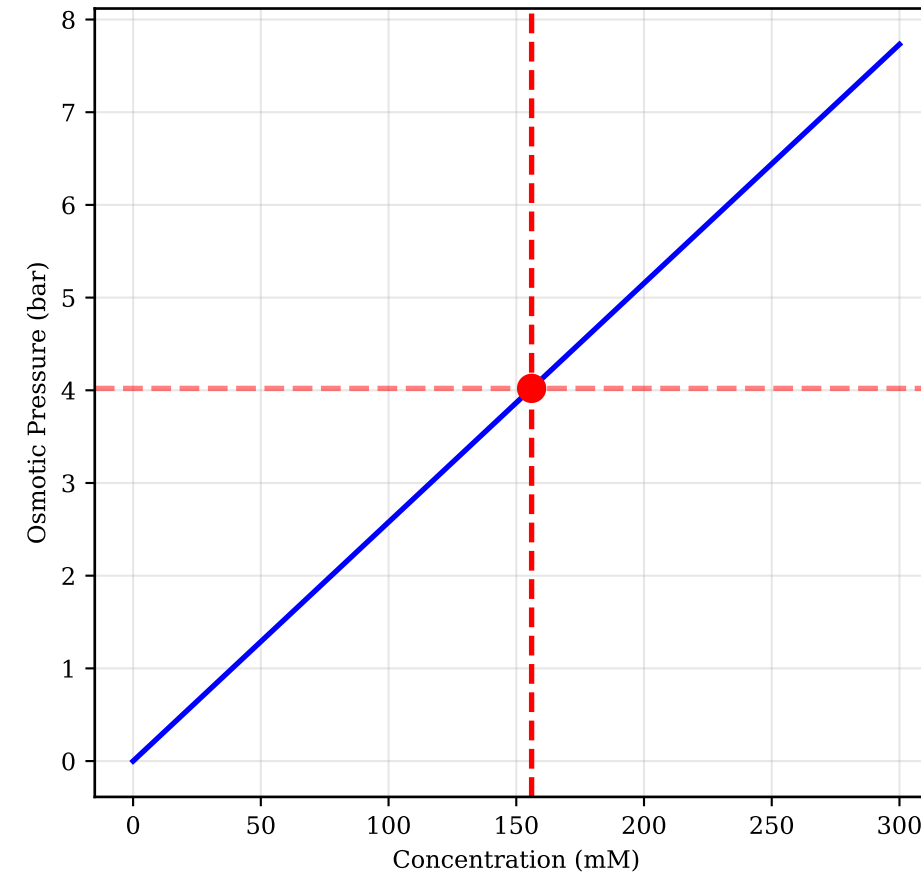
\Pi = cRT
