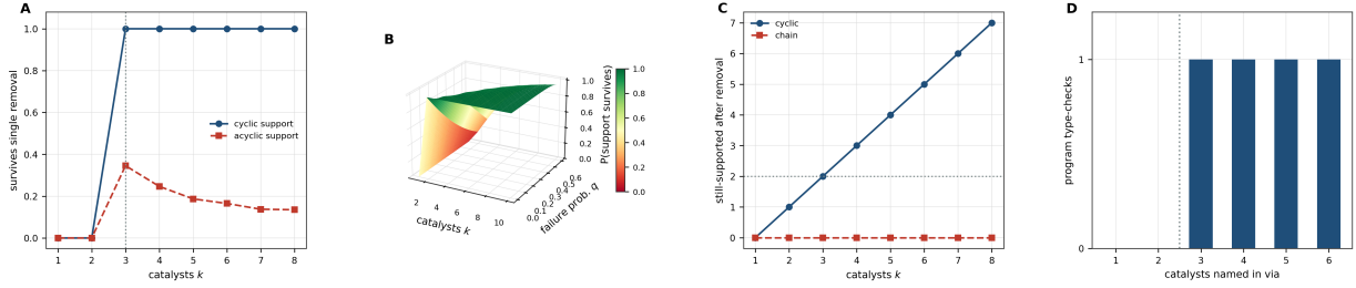
Figure 3: Robustness against the loss of a single source appears at three catalysts and not before, and the type checker enforces the boundary rather than recommending it. Panels (A)–(C) evaluate the combinatorics of support structures; panel (D) is measured from the implementation, by submitting programs to the type checker and recording what it accepts. (A) Probability that a conclusion survives removal of an arbitrary single catalyst, for cyclic and acyclic support structures, against the number of catalysts. Cyclic support jumps from 0 at k = 2 to 1 at k = 3 and stays there; acyclic support peaks at 0.34 and decays toward zero, never reaching robustness at any size. This is Theorem 5.2 and Theorem 5.3 together: no chain is robust however long, because its terminal member is licensed by nothing, and the shortest cycle compatible with robustness has length three. A 2-cycle fails not for want of evidence but for want of an arbiter—removing either member leaves the other supported by nothing. (B) Probability that at least two mutually supporting catalysts remain after independent per-catalyst failures, over k and the failure probability q . At q = 0.2 the probability rises from 0.640 at k = 2 to 0.896 at k = 3 and 0.993 at k = 5 ; at q = 0.4 the same k = 3 structure retains only 0.648. The third catalyst is the step that lifts the surface away from the failure plane, and the surface makes visible what the rule cannot promise: three unreliable catalysts are not equivalent to three reliable ones, and the rule constrains structure, not quality. (C) Number of catalysts still supported after one removal. A cycle retains k - 1 , rising linearly; a chain retains none at any k . The dotted line at two marks the minimum needed for mutual support to persist, which the cyclic case first clears at k = 3 . (D) Whether the type checker accepts a program naming k mutually independent catalysts. Programs at k = 1 and k = 2 are rejected by T-SEEK-COH; programs at k = 3 through 6 are accepted. The boundary is enforced at compile time and is not a convention a user may set aside. What the rule cannot do is verify the independence it requires (Theorem 5.4): three catalysts sharing an upstream data source or a common preprocessing step satisfy it while violating its intent, so the declaration is made visible in the source and left auditable rather than checked.
