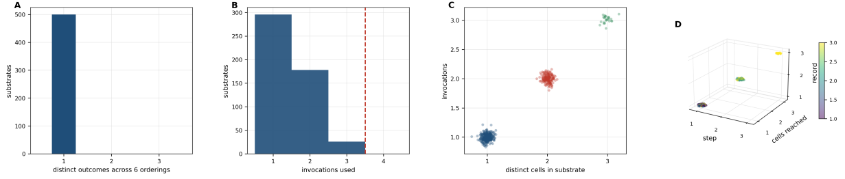
Figure 2: The metatheory holds on every evaluation tested, and the invocation count is exactly the number of destinations the substrate contains. 500 random substrates, each evaluated under all six orderings of the catalyst set—3000 evaluations—with outcomes compared by structural equality rather than by representative. (A) Distinct outcomes obtained across the six orderings, per substrate. Every substrate yields exactly one: there are no substrates in the two- or three-outcome bins. This is Theorem 6.7, and it holds because the reached-cell set is built by union, which is order-insensitive, while the closure rules branch only on that set’s cardinality. Non-determinism can therefore enter only through the substrate’s own responses, never through the language. (B) Invocations used per substrate against the bound |\Gamma_{\text{avail}}| = 3 marked in red. The distribution is supported entirely at or below the bound—296 substrates at one invocation, 178 at two, 26 at three, none above—confirming Theorem 6.8 with no exceptions. The strong skew toward a single invocation shows that closure is usually cheap: it costs the full registry only when the registry genuinely disagrees. (C) Invocations against the number of distinct cells the substrate contains. The two are equal on every substrate, giving three tight clusters on the diagonal with no off-diagonal mass. A seek therefore invokes exactly as many catalysts as there are distinct destinations to discover and stops—it does not exhaust the registry when the registry agrees, and does not stop early when it does not. (D) Record against step and cells reached, over every ordering of every substrate, coloured by the substrate’s cell count. Points lie only where record equals step, so each committed invocation advances the record by exactly one, and the cells-reached coordinate is non-decreasing along every trajectory. No configuration recurs at a smaller record, which is Theorem 6.6: a program’s provenance ordering is intrinsic to its own execution and needs no external timestamp.
