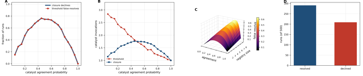
Figure 1: A threshold rule fails on exactly the runs where the evidence is contested, and the two rates coincide identically rather than approximately. Every point is measured by evaluating the same seek under the two termination rules on identical substrates and identical catalyst orderings, so the comparison isolates the stopping criterion and nothing else. The confident cell carries attained uncertainty 5.0 against a threshold of 10.0; the incompatible alternative carries 40.0 and never satisfies the threshold alone. (A) Fraction of runs on which closure declines, and fraction on which the threshold rule reports a single answer despite the evidence being split, against the probability that catalysts agree; 400 substrates at each of 20 levels. The two curves are equal to machine precision at every level—maximum absolute difference 0.0—which is why one is drawn heavy and the other dashed over it. The coincidence is not a coefficient to be estimated: whenever the reachable set contains more than one cell, some catalyst reaches the cell satisfying the threshold, and the threshold rule halts there by construction. On this substrate family the threshold rule is wrong on every contested run and on no others. The rate is non-monotone, peaking at 0.763 near even agreement and falling to 0.150 and 0.0 at the extremes, because unanimity—on either cell—leaves nothing contested. (B) Catalyst invocations paid by each rule. The threshold rule pays 2.84 invocations when agreement is low and 1.0 when it is high; closure peaks at 1.76 in the middle. The threshold rule is therefore cheapest exactly where it errs most, which is the economic shape of the failure mode: it stops early precisely when stopping early is unsafe. (C) False-resolve rate over agreement probability and registry size. The surface rises with registry size at fixed agreement, because each additional uninvoked catalyst is a further opportunity for an unconsulted source to disagree. Enlarging the registry—adding evidence—makes a threshold rule worse, which inverts the relationship an inquiry should have with its own resources. (D) Outcome split over 500 random substrates: 291 resolved, 209 declined. Both branches of Theorem 6.10 occur under ordinary substrate sampling. We report the split because a dichotomy theorem is compatible with one branch being unreachable in practice, and a language whose declination branch never fired would be a threshold rule wearing different syntax.
