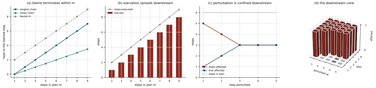
Figure 3: Blame: it terminates, and it only ever runs downstream. Plans of length m = 2 \dots 9 are executed with a starving first step and the blame chain is walked to its root; hop counts are traversal lengths recorded during the walk. (A) The longest and mean blame chain against plan length, with the m -hop bound of Theorem 5.13. The measured maximum is exactly m - 2 and the mean exactly (m - 2)/2 , both strictly under the bound at every length. The mechanism is that positions strictly decrease along a chain, so termination is not a budget but an arithmetic fact. (B) How much of each plan starves. Exactly m - 1 of m steps starve at every length: one step fails and every step below it inherits the failure, which is Theorem 5.9 read off the executed plans rather than argued. (C) A single perturbation applied at each position of one six-step plan. Perturbing step 1 affects 5 steps and first bites at 1; perturbing steps 3, 4 or 5 affects 3 and first bites at 3. The two series diverge because the first affected step is not the perturbed step once the perturbation lands inside a region already downstream of a common dependency. (D) The reachability cone the previous panel summarises: for each perturbation position i , which steps j can be affected. The filled cells lie on or below the diagonal only — nothing upstream of the perturbation is ever touched. That null could have failed: the sweep records reachability as computed from the executed dependency graph, not from a triangular structure that would make the shape true by construction.
