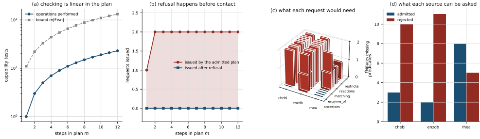
Figure 1: The static layer: checking is cheap, and refusal precedes contact. Every quantity is produced by running the checker and the executor over parsed plans against a local registry of three sources and thirteen predicates; no request leaves the machine, so a request issued is a counter the executor incremented and not an estimate. (A) Operations performed by the check against plan length for m = 1 \dots 12 . The measured count is exactly 2m - 1 against a declared bound of 11m , one per feature; the check is linear in m|\text{Feat}| as Theorem 4.5 requires, and the gap between the two lines is the constant the bound does not attempt to be tight about. (B) Requests actually issued, at every plan length rather than at one. The upper series is what the well-capable plan spends and the lower is what the same plan spends once its first step is pointed at a source that cannot answer it; Theorem 4.6 pins the lower series at exactly 0 for all twelve lengths. The upper series is 1 at m = 1 and then saturates at 2 : the chain starves after its second step, so the saving does not grow with m , and this caption declines to draw a curve that would suggest it does. (C) For each of 39 source–predicate pairs, the number of declared features the request would still need. The height is the integer the checker computed, so the bars are drawn as bars: a surface would interpolate a step function through values it never takes. Zero (blue) means admissible, and 2 (red) means two features short. (D) The same 39 pairs resolved into admitted and rejected counts per source. The three sources are unequal by construction — chebi admits 3 of 13, enzdb 2, rhea 8 — and it is that inequality, not the checker, that decides which plans can be written at all. Under Theorem 3.16 this figure records what each source declares ; an over-declaration would be invisible here, which is the asymmetry the prototype cannot test away.
