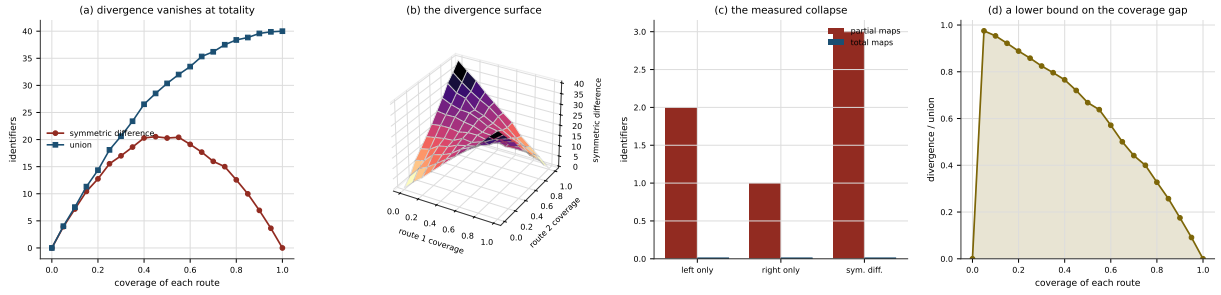
Figure 5: Two routes: divergence is a coverage gap, and it collapses under totality. Two independent routes between the same endpoints are resolved at controlled coverage; the symmetric difference is computed on realised identifier sets, and the interpretation of Theorem 6.11(b) is fixed before any number is read. (A) Symmetric difference and union as both routes are made more total, 21 coverage levels. The divergence rises to a maximum of 20.3 identifiers near coverage 0.4 and then falls back to exactly 0 at coverage 1.0, while the union climbs monotonically to 40. The non-monotone shape is the substance: divergence is small when both routes see little and small again when both see everything, and it is largest in between. (B) The same quantity over independent coverage for the two routes, 121 cells. The surface carries a ridge along the diagonal, peaking at 20.6 where both routes cover half. Only 2 of 121 cells are exactly zero, and both lie at the corners where the two routes agree trivially. (C) The measured collapse from the fixture. With partial maps the routes differ on 3 identifiers — 2 resolved only by the direct route, 1 only by the indirect — out of a union of 8. With both maps made total, all three counts are exactly 0; the thick rules mark those measured zeros so they cannot be mistaken for an absent series. (D) Divergence as a fraction of the union, which is the form in which the claim is actually usable. The fraction peaks near 0.6 and returns to 0 at totality. Per Theorem 6.11(b) this is a lower bound on the correspondences at least one route fails to resolve, and not a count of errors: neither route contradicts the other anywhere in this sweep, and nothing here licenses reading a divergence as one route being wrong.
