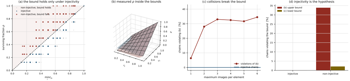
Figure 4: Injectivity is the hypothesis, not a convenience of the proof. Chains are drawn over 8-element supports at domain probability 0.8 and at most 3 images per element; injective chains are constructed rather than rejection-sampled, so the two populations are matched in everything except the property under test. (A) Surviving fraction \rho against \min_i r_{\mu_i} for 1200 injective and 1158 non-injective chains. Every injective chain lies on or below the diagonal, as Theorem 6.4(b) requires. Of the non-injective chains, 315 (27.2%) lie strictly above it and are drawn alone in the alarm colour; the remainder are greyed, because a non-injective chain that happens to respect the bound is not evidence either way. The shaded wedge above the diagonal is the region the theorem forbids under its hypothesis, and it is populated. (B) Measured \rho (wireframe) between the upper bound of (b) and the lower bound of (c) over an 8 \times 8 grid in (r_1, r_2) , 64 cells. The measured value touches the upper sheet in 8 cells and never crosses either sheet. The vertical separation reaches 0.253 above and 0.247 below, and per Theorem 6.6 that separation is not slack to be tightened: the two bounds answer different questions. (C) Violation rate of (b) against how non-injective the chain is, 600 trials at each image cap. At one image per element the rate is 6.3% — not zero, because capping images at one does not by itself forbid two elements sharing an image — rising to 28–34.5% once two or more images are allowed. The flat blue line is the constructed-injective control at exactly 0; without it the red curve would have no floor to be read against, and the 6.3% would look like noise rather than residual collision. (D) Both bounds against both populations at n = 5000 each. Injective chains violate the upper bound 0 times and the lower bound 0 times; non-injective chains violate the upper 1694 times (33.9%) and the lower 102 times (2.0%). The four bars are the whole of Theorem 6.5: two zeros that could have been non-zero, beside two non-zeros that could have been zero.
