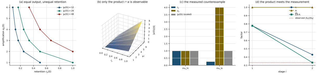
Figure 6: Retention and amplification are independent, and output size sees only their product. Retention r_\mu(S) = |S \cap \text{dom } \mu|/|S| and amplification a_\mu(S) = |\mu(S)|/|S \cap \text{dom } \mu| are computed on realised sets from executed maps; 144 cells sweep the pair. (A) Iso-cardinality families: every point on one curve produces the same |\mu(S)| . At |\mu(S)| = 12 the retention ranges over 0.083–0.5 while the amplification ranges over 1–6, a spread of 6.0; at |\mu(S)| = 24 the same spread holds at retentions 0.167–1.0. Equal output size is compatible with a sixfold difference in how much of the input survived. (B) The observable ratio |\mu(S)|/|S| = r \cdot a over the (r, a) plane, with the level curves at 0.5, 1 and 2 projected onto the floor. The surface is a product, so its level sets are hyperbolae and every point on one is indistinguishable from the outside: this is exactly what Theorem 6.3 claims cannot be undone by measuring |\mu(S)| more carefully. (C) The measured counterexample, executed rather than constructed on paper. Two maps over the same 8-element input both emit 8 identifiers; mu_hi has r = 1.00 , a = 1.0 and mu_lo has r = 0.25 , a = 4.0 — a retention ratio of 4.0 at identical output cardinality and identical product 1.0. The grey series is output size, scaled, and its flatness is the point. (D) The factorisation of Theorem 6.4(a) along a measured two-stage chain. Stage retentions are 0.778 and 0.429 with both amplifications 1.0; the running product reaches 0.333 and the observed |S_k|/|S_0| is 0.333 to the last recorded digit. This chain is not injective, and part (a) holds anyway — which is why (a) is stated unconditionally and (b) and (c) are not.
