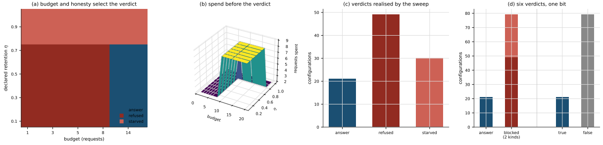
Figure 2: The verdict layer: six outcomes, one observable bit. A 10 \times 10 sweep executes the same plan across ten budgets B \in \{1, 2, 3, 4, 5, 6, 8, 10, 14, 20\} and ten declared-honesty levels \eta \in \{0.1 \dots 1.0\} , giving 100 executed plans; the verdict in each cell is the one the ordered rules (R1)–(R6) of Theorem 5.7 returned. (A) The verdict attained in each cell. Of the 100 executions, 21 answer, 49 refuse and 30 starve, and answer appears only at budgets 10, 14 and 20. The budget axis is geometric and is labelled by value rather than by position, because drawing \{1 \dots 20\} on a linear extent would misstate where the transition sits. (B) Requests spent before the verdict was returned. The spend is single-valued within each verdict — 9.0 for answer , 2.0 for refused , 2.0 for starved — so the plot has three levels and not a cloud. The refused here is budget exhaustion and costs 2.0 requests; it is not the static ill-capability refusal of Figure 1(B), which costs 0. The two share a name and nothing else, and no figure in this paper should be read as reconciling them. (C) The verdicts the sweep realises from named plans, with the blocker each carries. All six of Theorem 5.7 occur, with blockers model , engine , corpus and budget for the four blocked kinds and none for the two that are not blocked. (D) The collapse of Theorem 5.8. Across the sweep, 21 executions carry the true bit and 79 the false one; the five non- answer kinds are distinct verdicts with distinct blockers and identical payload size 0, so a caller reading only success or failure cannot separate them. Theorem 1.2 is what makes this a collapse rather than a loss: a payload accompanies answer alone, so there is nothing else for the bit to have carried.
