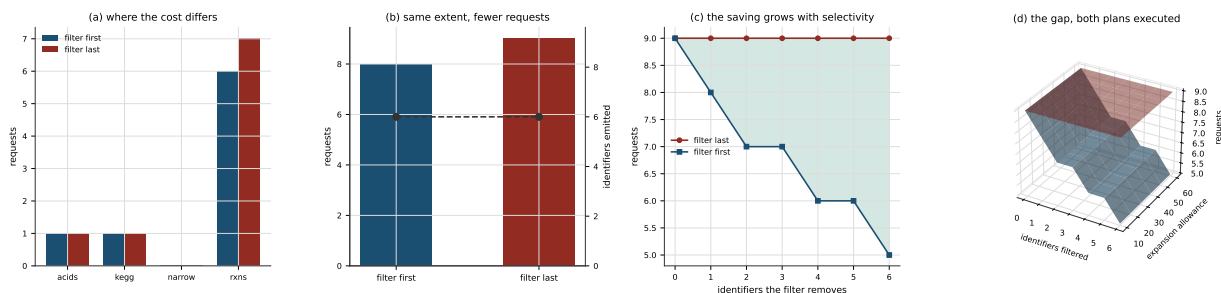
Figure 8: Ordering: the same extent at a different price. Two plans containing the same four steps in two orders are parsed, checked and executed; every request count below is a counter the executor incremented, and the closed-form cost model that also exists in the sweep is deliberately not plotted anywhere in this figure. (A) Requests spent per step by the two orderings. The steps acids and kegg cost 1 each in both plans; the difference is entirely in the last two, where filtering first makes rxns cost 6 and filtering last makes it cost 7. No step is cheaper under the worse ordering, which is what makes the comparison a saving rather than a trade. (B) Totals. Both plans emit the same six identifiers — RHEA:100 through RHEA:105 , set-equal and not merely equal in count — at 8.0 and 9.0 requests. The dashed coverage line is flat by measurement, and if it were not, the request comparison beside it would mean nothing. (C) Both orderings executed as the filter is made more selective, at the expansion allowance the shipped plans use. Requests under filter-last stay pinned at 9.0 regardless of selectivity, while filter-first falls 9.0 \rightarrow 5.0 as the filter removes 0 \rightarrow 6 identifiers. The measured series has step structure — flat across 2 \rightarrow 3 and again across 4 \rightarrow 5 — which a smooth cost model would have drawn as a straight line. (D) The two measured surfaces over filter size and expansion allowance, 42 executed plans. The sheets touch at zero selectivity and separate as the filter bites, with a maximum measured saving of 4 requests. Coverage was checked equal in all 42 cells; per Theorem 6.9 the saving is a cost difference and never an extent difference, and the sweep records no cell where that failed.
