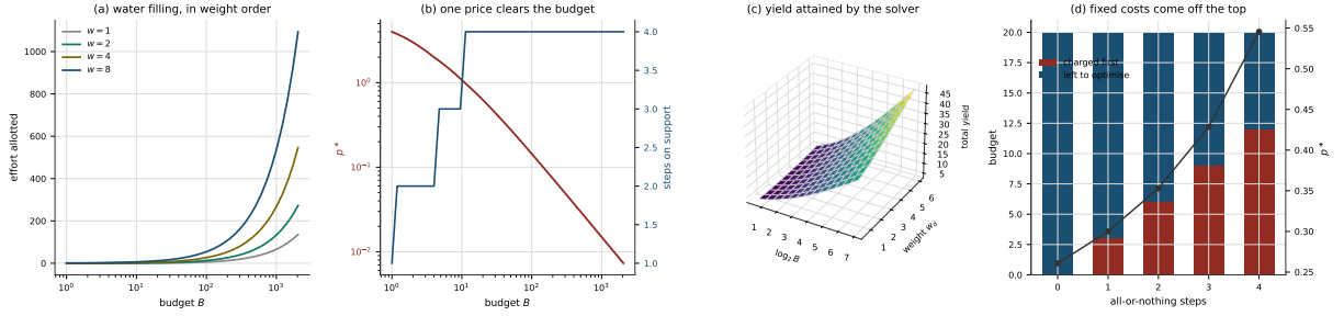
Figure 7: Allocation: one shadow price clears the budget, and fixed costs are charged before it. The allocator of Theorem 7.3 is solved at 45 budgets spanning B = 1 to 2048 over four steps of weight 1, 2, 4, 8; every plotted effort is a solved primal variable and every price a solved dual. (A) Effort allotted to each step as the budget grows, on a logarithmic budget axis. Steps enter in weight order and not together: at B = 1 only the heaviest step is funded, at B = 4 two are, and all four are on support from B = 16 upward. Water filling is visible as the staggered onset, which no single-budget summary of the allocator would show. (B) The shadow price p^* and the size of the support against the budget, with the price on logarithmic axes. p^* falls monotonically from 4.00 to 7.31 \times 10^{-3} across the sweep while the support rises from 1 to 4 and then stops; the kinks in the price are exactly the budgets at which a step enters. The maximum KKT residual over all 45 solves is 1.11 \times 10^{-16} , which is machine epsilon rather than a tolerance that was chosen. (C) Total yield over budget and the weight of the fourth step, 168 solved allocations. The surface is concave in \log_2 B at every weight, and the yield rises from 5.55 at B = 1 to 97.34 at B = 2048 . (D) What happens when steps carry an all-or-nothing or fixed cost: those are charged first and the optimiser gets what remains. As the number of such steps goes 0 \rightarrow 4 , the charged-first amount rises 0 \rightarrow 12 and the optimised budget falls 20 \rightarrow 8 ; the price rises with it, 0.261 \rightarrow 0.545 . The rising price is the honest report that the same total budget buys strictly less once part of it is spent before the optimisation can see it.
