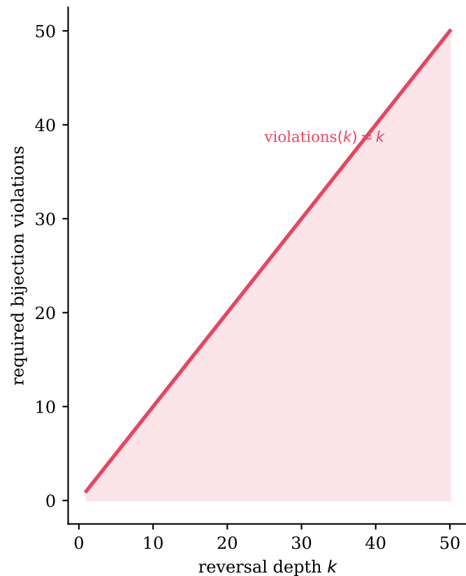
Violations = k for Depth- k Reversal
