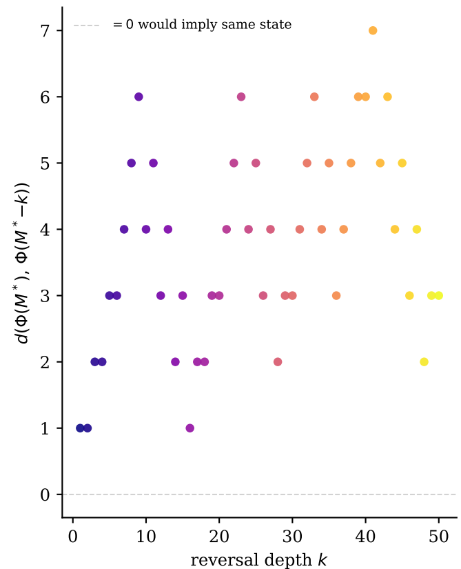
State Distance > 0 for All k \geq 1
