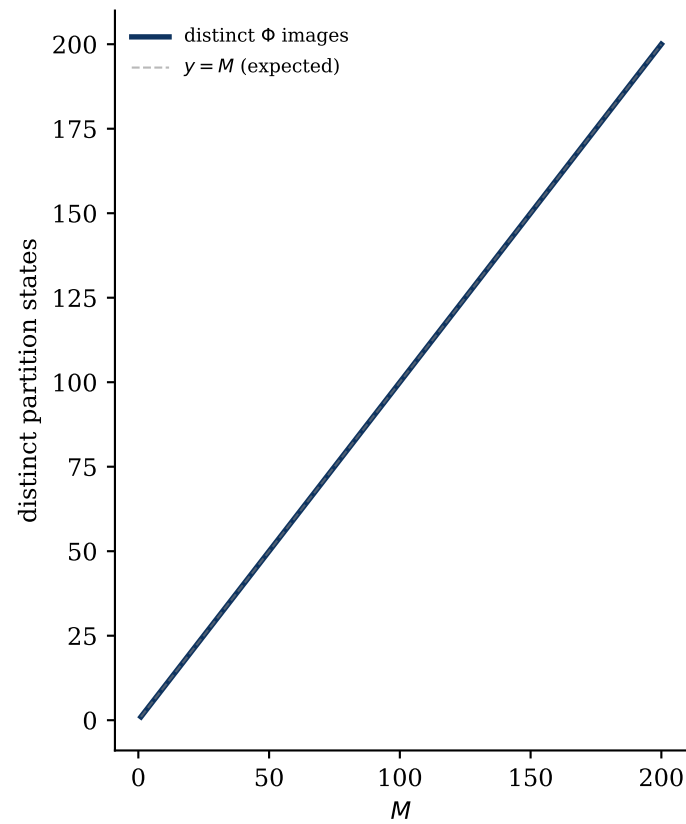
Injectivity Confirmed: All M Unique
