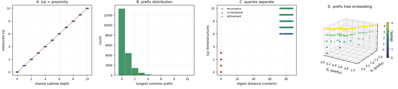
Figure 8: Prefix is Proximity and the Paired Content–Time Label. (A) Measured longest-common-prefix on the linear y -axis versus the constructed shared-subtree depth on the linear x -axis (steelblue points, jittered, 4000 leaf pairs in a depth-10 base-3 work-tree), with the identity diagonal marked (crimson dashed). Every point lies on the diagonal: the longest common prefix equals the depth of the leaves’ lowest common ancestor, the empirical content of Theorem 9.8(i) (prefix is proximity). (B) Distribution of the longest common prefix over 20,000 random leaf pairs in a base-3 depth-10 tree (green bars, white edges). The mass concentrates at small prefixes, the geometric base- b profile expected when unrelated leaves share short prefixes; it is the background against which a large prefix certifies genuine structural proximity (Theorem 9.8). (C) The three relatedness queries in the (digest distance, lcp) plane: recurrence (crimson, digest distance 0, small lcp), co-temporality (steelblue, large digest distance, large lcp), and refinement (green, large digest distance, large lcp), 300 points each. The queries occupy disjoint regions, the empirical content of Theorem 9.11 (decidable queries): each is decided by a constant number of comparisons on the paired label. (D) Three-dimensional embedding of a depth-4 base-3 address tree: each node placed at (S_k, S_t) from the base-3 digit-path expansion of its address, height equal to tree depth, points coloured by depth on the viridis scale, viewing angle elevation 20^\circ azimuth -58^\circ . Nodes sharing an address prefix cluster spatially and stack by depth, the geometric realisation of Theorem 9.8: shared prefix is shared structural position, the relatedness face of the paired label (Construction 9.10).
