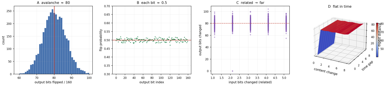
Figure 7: Avalanche and Time-Blindness of a Content Digest. (A) Distribution of the output Hamming distance (out of 160 SHA-1 bits) induced by a single input-bit flip, over 4000 random 32-byte inputs (steelblue bars, white edges), with the half-width value 80 marked (crimson vertical line). The distribution concentrates at \approx 80 bits: a minimal (maximally related) input difference produces a near-half output difference, the empirical content of Theorem 9.2 (Label orthogonality) via the strict avalanche criterion. (B) Per-output-bit flip probability on the linear y -axis versus output bit index 0 to 159 on the linear x -axis (green points), measured over 3000 single-bit input flips, with the value 0.5 marked (crimson line) and the y -axis restricted to [0.3, 0.7] . Every output bit flips with probability \approx 0.5 , the strict avalanche criterion that makes a digest identity-faithful and, by Theorem 9.2, relatedness-destroying. (C) Output bits changed on the linear y -axis versus number of input bits changed (1 to 5, jittered) on the linear x -axis (purple points, 1500 trials), with the half-width 80 marked (crimson dashed). The output difference is \approx 80 regardless of how few input bits differ: related inputs map to maximally distant digests (Corollary 9.3). (D) Three-dimensional surface of mean digest distance over content change (0 to 8 input bits flipped) and time gap (0 to 8 trajectory-count units), coolwarm colourmap, viewing angle elevation 22^\circ azimuth -62^\circ . The surface rises with content change but is flat along the time-gap axis: the digest is a function of content alone, the empirical content of Theorem 9.5 (Time-blindness)—temporal proximity is invisible to a content hash.
