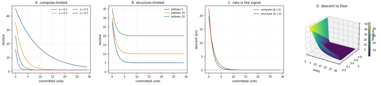
Figure 4: Runtime Diagnosis: Compute-Limited versus Structure-Limited from the Residue Stream Alone. (A) Residue on the linear y -axis versus committed units on the linear x -axis for four compute-limited streams with geometric descent rates \kappa \in \{0.1, 0.3, 0.5, 0.7\} (steelblue, orange, green, purple); the floor is marked (crimson dashed). Each stream descends with strictly positive rate \Delta(n) > 0 toward the floor, the compute-limited regime of Definition 6.2 and Theorem 6.3. (B) Residue on the linear y -axis versus committed units on the linear x -axis for three structure-limited streams that plateau above the floor at levels \{5, 10, 20\} (steelblue, orange, green); the floor is marked (crimson dashed). After an initial descent the rate \Delta(n) \rightarrow 0 while residue remains strictly above the floor, the structure-limited regime of Definition 6.2. (C) Descent rate \Delta(n) on the linear y -axis versus committed units on the linear x -axis for a representative compute-limited stream (green, \Delta > 0 sustained) and a structure-limited stream (crimson, \Delta \rightarrow 0 ), with the zero line marked (grey). The sign of \Delta(n) alone separates the two regimes, the decidability claim of Theorem 6.3: limit type is read from the residue stream without any running-time estimate. (D) Three-dimensional surface of residue \rho = \beta + (50 - \beta)(1 - \kappa)^n over committed units n \in [0, 30] and descent rate \kappa \in [0.05, 0.9] , viridis colourmap, viewing angle elevation 24^\circ azimuth -58^\circ . The surface descends to the floor for every \kappa , the family of compute-limited convergences whose strictly positive \Delta marks them feedable (Theorem 6.3).
