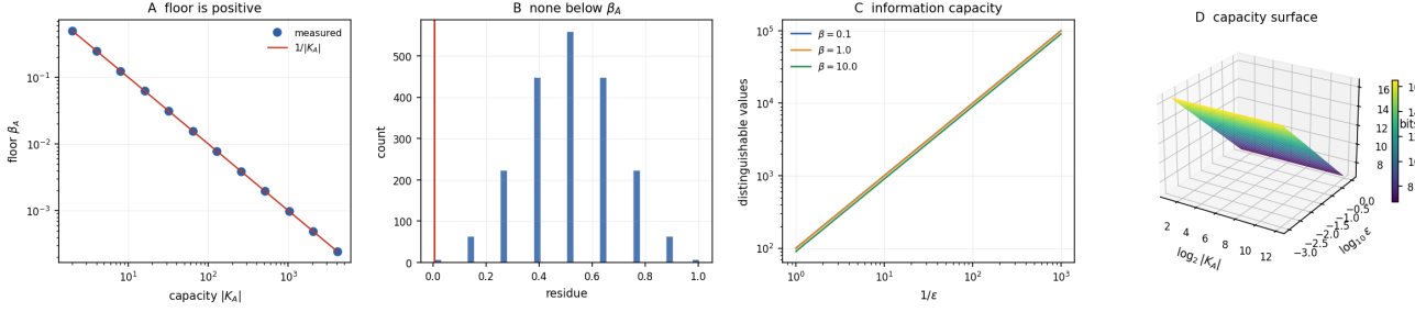
Figure 1: The Residue Floor and the Information Capacity of the Residue Scale. (A) Measured diagonal floor \beta_A on the logarithmic y -axis versus agent capacity |K_A| on the logarithmic x -axis for twelve capacities |K_A| \in \{2, 4, 8, \dots, 4096\} . Steelblue circles are the floor read from a bounded agent whose encoder collapses |K_A| \cdot 8 candidates onto |K_A| internal states; the crimson line is the prediction \beta_A = 1/|K_A| . The measured floor coincides with 1/|K_A| to machine precision at every capacity and is strictly positive throughout, the empirical content of Theorem 3.1 (Residue Floor): a bounded agent cannot resolve a candidate below a strictly positive floor. (B) Distribution of the residue read over all |K_A| \cdot 8 candidates at capacity |K_A| = 256 (steelblue bars, white edges), with the floor \beta_A = 1/256 marked (crimson vertical line). The histogram is supported entirely at and above the floor; no candidate is read below it, confirming the no-candidate-below-floor clause of Theorem 3.1. (C) Number of distinguishable residue values on the logarithmic y -axis versus inverse precision 1/\epsilon on the logarithmic x -axis, for floors \beta \in \{0.1, 1.0, 10.0\} (steelblue, orange, green) over \epsilon \in [10^{-3}, 1] . Each curve is the predicted bound \lceil (U - \beta)/\epsilon \rceil with U = 100 ; the distinguishable-value count rises linearly in 1/\epsilon , the content of Theorem 3.3 (Information capacity). (D) Three-dimensional surface of the residue-scale information content \log_2((U - \beta)/\epsilon) over \log_2 |K_A| \in [1, 12] and \log_{10} \epsilon \in [-3, 0] , with \beta = 1/|K_A| and U = 100 , viridis colourmap, viewing angle elevation 24^\circ azimuth -58^\circ . The surface is strictly positive throughout and rises as precision sharpens, displaying the sizing law of Theorem 3.3: distinguishing residue at precision \epsilon demands the indicated bits of representational capacity.
