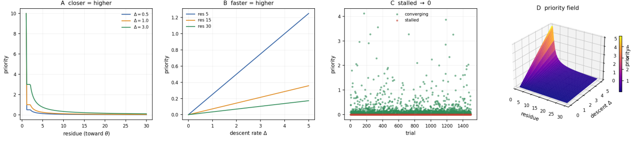
Figure 5: Residue Priority and Scheduler Soundness. (A) Priority P(\tau) on the linear y -axis versus residue (approaching the threshold \theta ) on the linear x -axis for descent rates \Delta \in \{0.5, 1.0, 3.0\} (steelblue, orange, green), clipped at 10. Priority rises as a task approaches its threshold, the closeness term of Definition 7.2: a nearly-done task is worth finishing. (B) Priority P(\tau) on the linear y -axis versus descent rate \Delta on the linear x -axis for residues \{5, 15, 30\} (steelblue, orange, green). Priority rises linearly in the descent rate, the rate term of Definition 7.2: a fast-converging task is worth advancing. (C) Priority on the linear y -axis versus trial index on the linear x -axis for 1500 randomly drawn task pairs: converging tasks (green, \Delta \in [0.01, 5] ) and stalled tasks (crimson, \Delta = 0 ). Every stalled task has priority 0 and none out-prioritises a converging task, the empirical content of Theorem 7.4 (Priority-rule soundness): a stalled task is never fed. (D) Three-dimensional priority field P = \Delta / \max(\rho - \theta, \beta_A) over residue \rho \in [1.01, 30] and descent rate \Delta \in [0, 5] (clipped at 5), \theta = 1 , plasma colourmap, viewing angle elevation 26^\circ azimuth -56^\circ . Priority is zero along the \Delta = 0 edge (stalled) and grows toward the high-rate, low-residue corner (converging and close), the geometric realisation of Definition 7.2 and Theorem 7.4.
