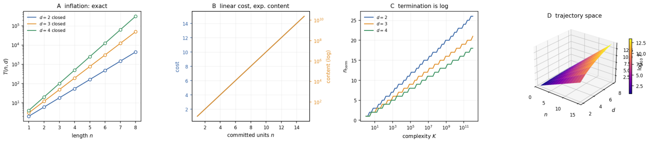
Figure 3: Trajectory Inflation and the Logarithmic Termination Bound. (A) Distinguishable work-trajectory count T(n, d) on the logarithmic y -axis versus length n \in \{1, \dots, 8\} on the linear x -axis for d \in \{2, 3, 4\} (steelblue, orange, green). Solid lines are the closed form T(n, d) = d(d+1)^{n-1} ; open circles are the direct enumeration of compositions of n times d -fold type labellings. The two coincide at every (n, d) —e.g. T(8, 4) = 1,399,680 —the empirical content of Theorem 5.3 (Trajectory inflation). (B) Dual-axis comparison for d = 4 : cumulative cost (steelblue, left linear axis) and distinguishable content T(n, d) (orange, right logarithmic axis) versus committed units n \in \{1, \dots, 15\} . Cost grows linearly while content grows exponentially, the asymmetry of Remark 5.7: linear cost, exponential content. (C) Termination unit count n_{\text{term}}(K, d) on the linear y -axis versus categorical complexity K on the logarithmic x -axis for d \in \{2, 3, 4\} (steelblue, orange, green), K \in [1, 10^{12}] . Each curve is logarithmic in K , e.g. n_{\text{term}}(10^{12}, 3) = 16 ; the content of Theorem 5.6 (Logarithmic termination bound). (D) Three-dimensional surface of \log_{10} T(n, d) over length n \in \{1, \dots, 15\} and type count d \in \{2, \dots, 8\} , plasma colourmap, viewing angle elevation 26^\circ azimuth -52^\circ . The surface rises exponentially in both n and d , the trajectory-space inflation that makes content-bounded termination logarithmic (Theorems 5.3, 5.6).
