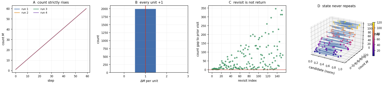
Figure 2: Strict Monotonicity of the Trajectory Count: an Undo is a Forward Unit. (A) Trajectory count M on the linear y -axis versus committed step on the linear x -axis for four independent 60-step runs (steelblue, orange, green, purple), each with a 30% fraction of “undo” units that restore a prior candidate. The crimson dashed line is the ideal M = \text{step} . Every run rises strictly and lies exactly on the diagonal, the empirical content of Theorem 4.2 (Strict monotonicity): each work unit, undo or not, increments the count. (B) Distribution of the per-unit increment \Delta M over a 2000-step run including undo operations (steelblue bars, white edges), with the value 1 marked (crimson vertical line). All mass sits at \Delta M = 1 : the count never decrements and never jumps, confirming that an undo is itself a counted forward unit. (C) Count gap between successive visits of the same candidate on the linear y -axis versus revisit index on the linear x -axis (green points), over a 400-step run with 40% undo. Every gap is strictly positive (all points above the crimson line at 0): a revisited candidate is reached at a strictly larger count, so it is a new state, the content of Corollary 4.3 (no return). (D) Three-dimensional state path (candidate (normalised), M , step) for a 120-step run with 35% undo, points coloured by count on the plasma scale, viewing angle elevation 22^\circ azimuth -60^\circ . The path advances monotonically in the count axis and never returns to a prior (x, M) state even where the candidate axis repeats, the geometric realisation of Theorem 4.2 and Corollary 4.3: resemblance of candidate is never identity of state.
