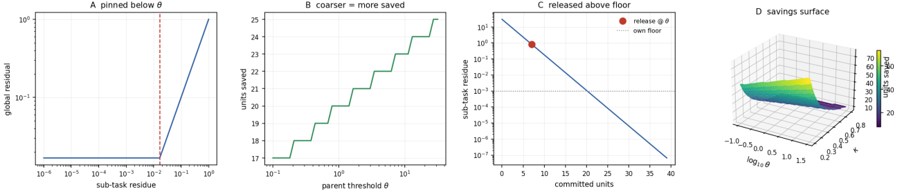
Figure 6: Sufficiency Stopping: a Sub-Task Released Above its Own Floor. (A) Global residual on the logarithmic y -axis versus sub-task residue on the logarithmic x -axis, with the parent threshold \theta = 1/60 marked (crimson dashed), over sub-task residues [10^{-6}, 1] . The global residual equals \max(\theta, \rho_{\text{sub}}) and is pinned at \theta once the sub-task crosses the threshold, the empirical content of Theorem 8.2: reducing the sub-task below \theta does not improve the global residual. (B) Committed units saved on the linear y -axis versus parent threshold \theta on the logarithmic x -axis (green), for geometric descent \kappa = 0.5 from start 50 to a sub-task floor 10^{-6} . The saved-unit count grows as the parent threshold coarsens, quantifying the cost spared by releasing at \theta rather than the sub-task’s own floor (Theorem 8.2, Example 8.3). (C) Sub-task residue on the logarithmic y -axis versus committed units on the linear x -axis (steelblue), with the release point at \theta = 1 marked (crimson circle) and the sub-task’s own floor at 10^{-3} marked (grey dotted). The task is released at \theta , strictly above its own attainable floor; the residue it could still reduce is never computed, the content of Theorem 8.2. (D) Three-dimensional surface of committed units saved over \log_{10} \theta \in [-1, 1.5] and descent rate \kappa \in [0.2, 0.8] (closed-form geometric, start 50, sub-task floor 10^{-6} ), viridis colourmap, viewing angle elevation 24^\circ azimuth -60^\circ . Savings grow as the parent floor coarsens and as descent slows, the surface form of the sufficiency-stopping economy (Theorem 8.2).
