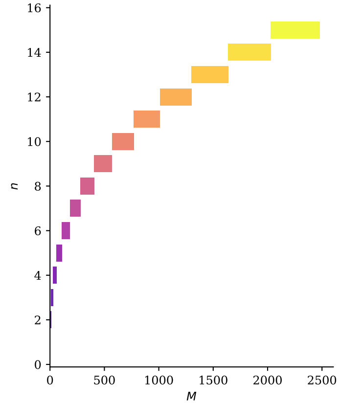
Level Boundaries
