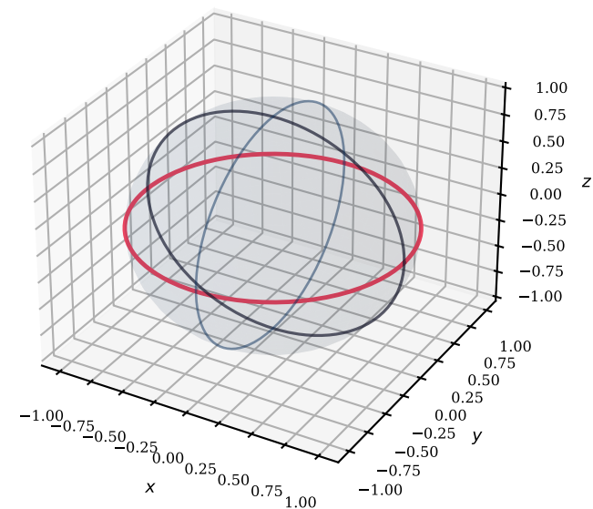
SO(3) Orbit Space
