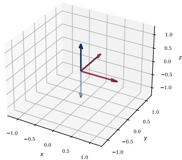
Axis Exchange \in SO(3)
