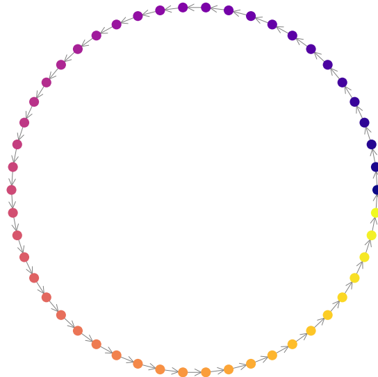
Cyclic Successor \sigma
