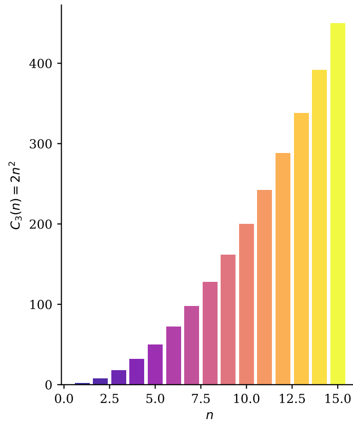
Level Sizes 2n^2
