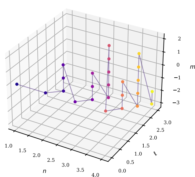
Trajectory in (n, \ell, m)
