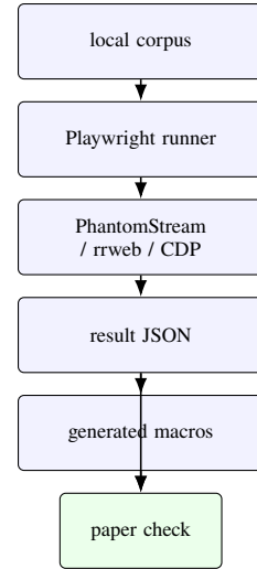
Fig. 3. Benchmark-to-paper pipeline. The paper imports generated result macros; the validator fails if required metrics are missing, non-finite, or mismatched.
