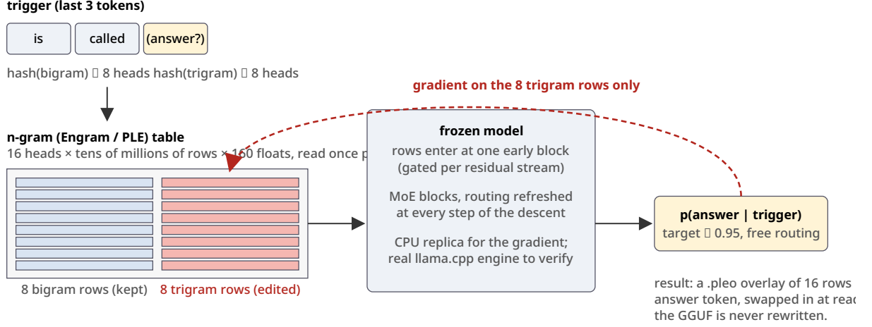
Figure 1: The trigger’s last three tokens are hashed into 16 rows of the table, 8 keyed by the bigram and 8 by the trigram. Only the 8 trigram rows receive gradient. The rows enter the frozen model at one early block; the loss is the answer’s log-probability at the output, under expert routing refreshed at each step. The result is a .pleo overlay swapped in at read time; the GGUF is never rewritten.
