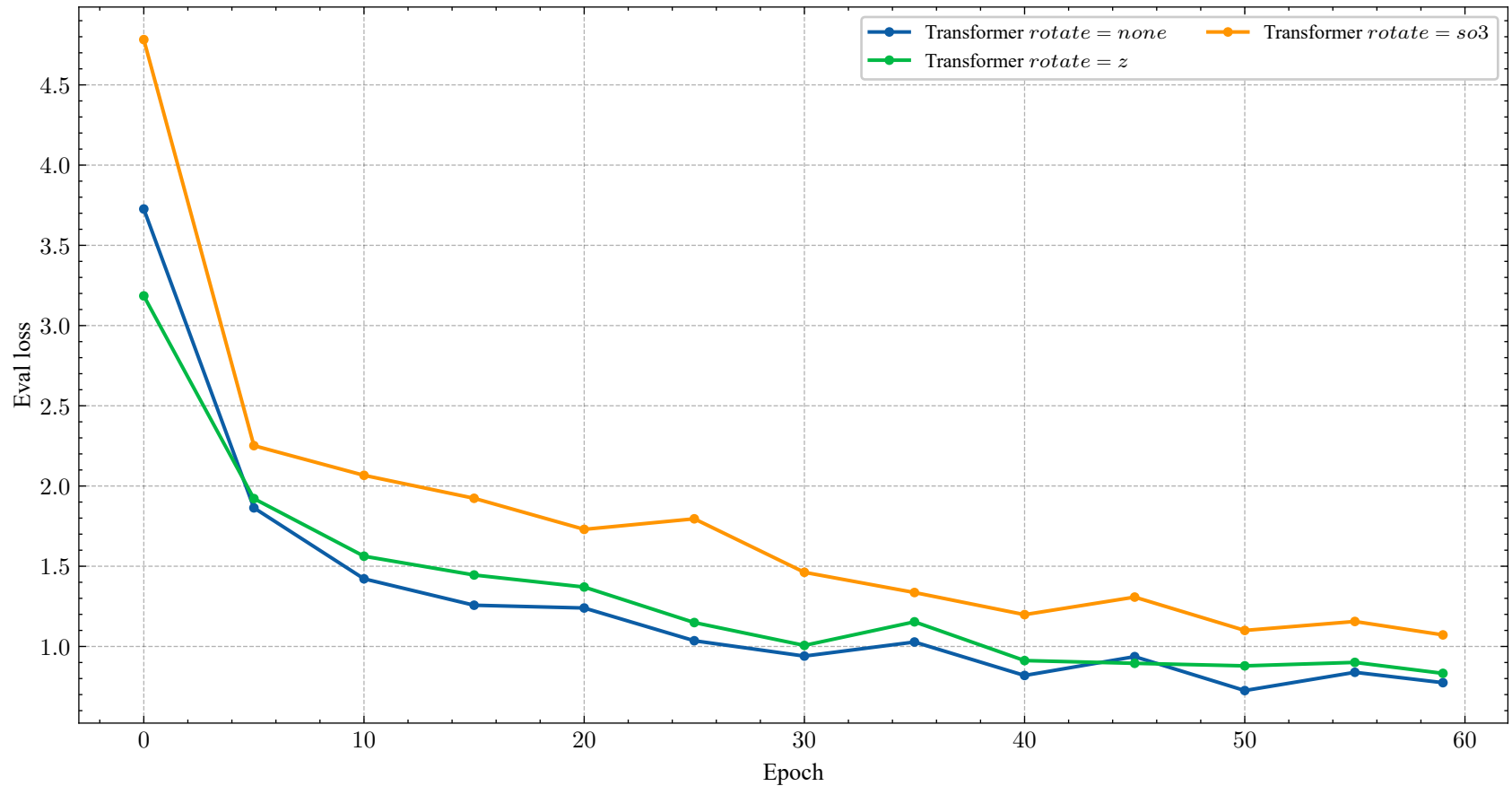
Eval loss over training epochs
