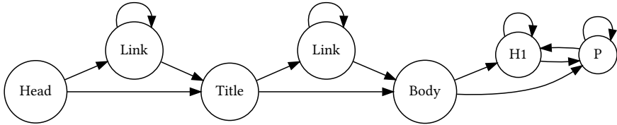
Figure 14: The HTML API protocol
