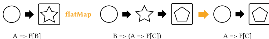
Figure 25: Type chart for flatMap applied to Check
