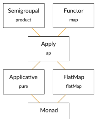
Figure 11: Monad type class hierarchy
