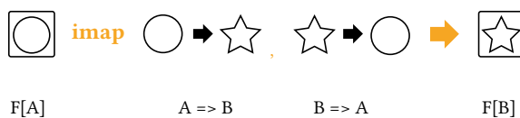
Figure 6: Type chart: the imap method
