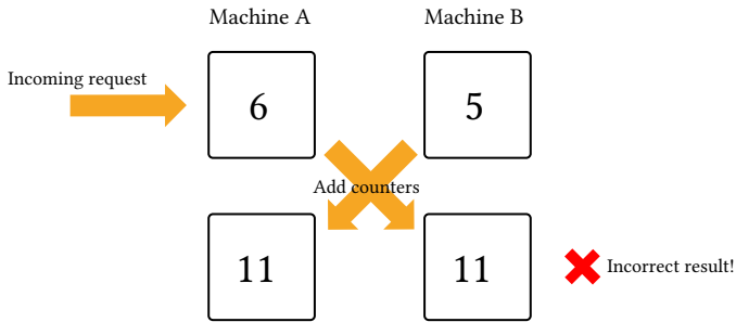
Figure 29: Simple counters: second round of requests and (incorrect) reconciliation
