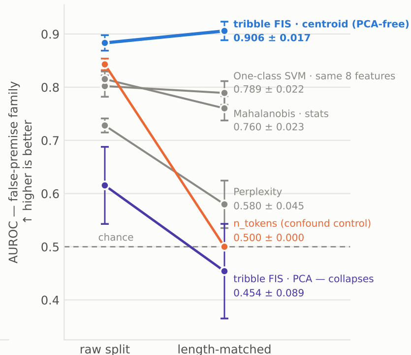
B • Controlling for answer length (10 seeds, mean \pm std)
