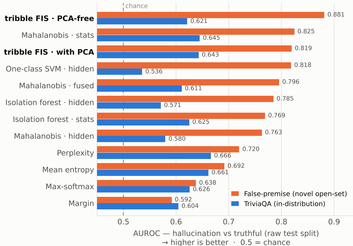
A • Detector comparison — raw split
