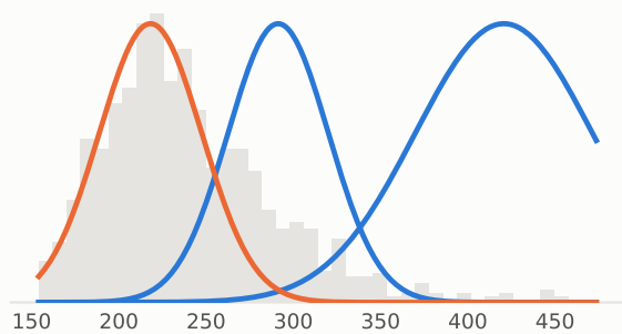
L28_dist
