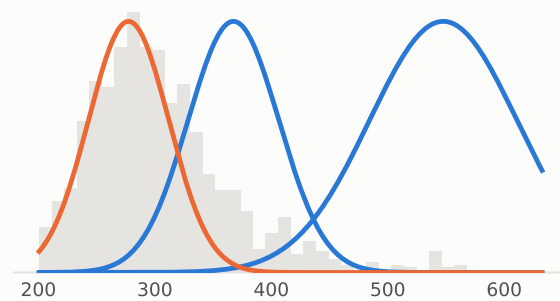
L30_dist
