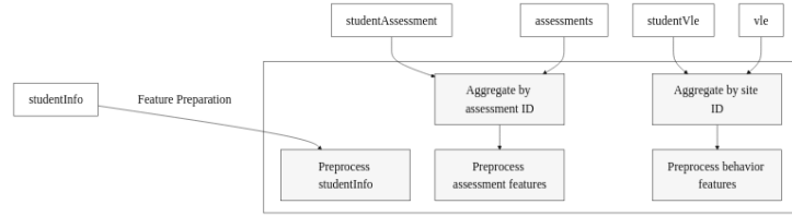
Fig. 2: Preprocessing pipeline (Stage 2): feature preparation.
