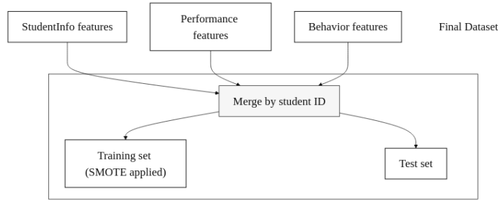
Fig. 4: Preprocessing pipeline (Stage 4): final dataset construction.
