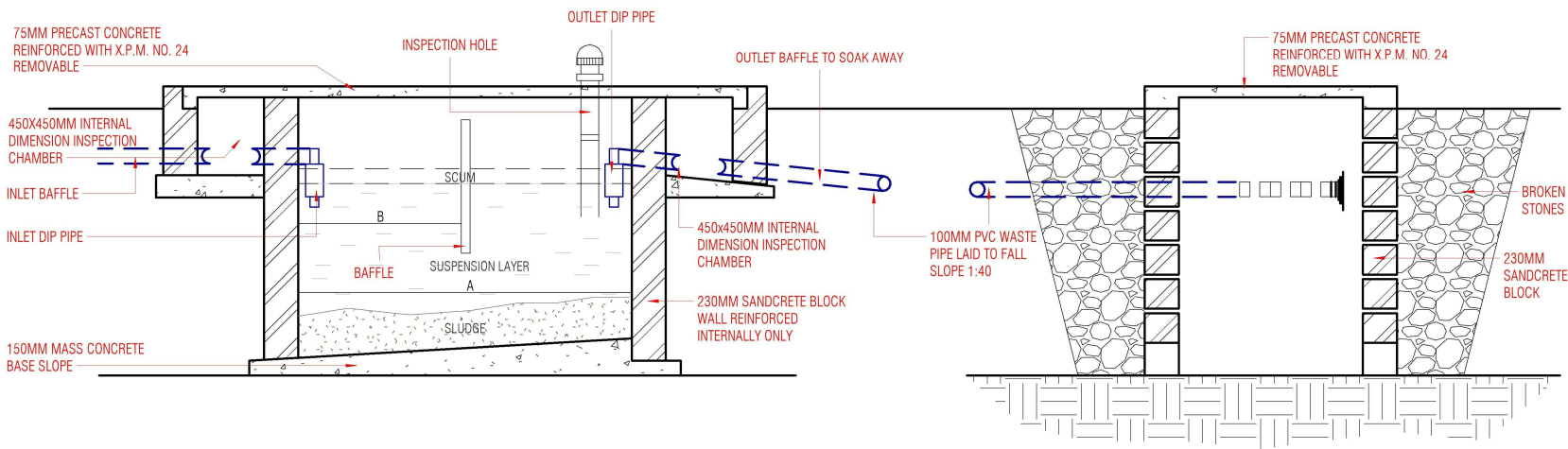
SEPTIC TANK / SOAK AWAY SECTION 1 1 : 50
