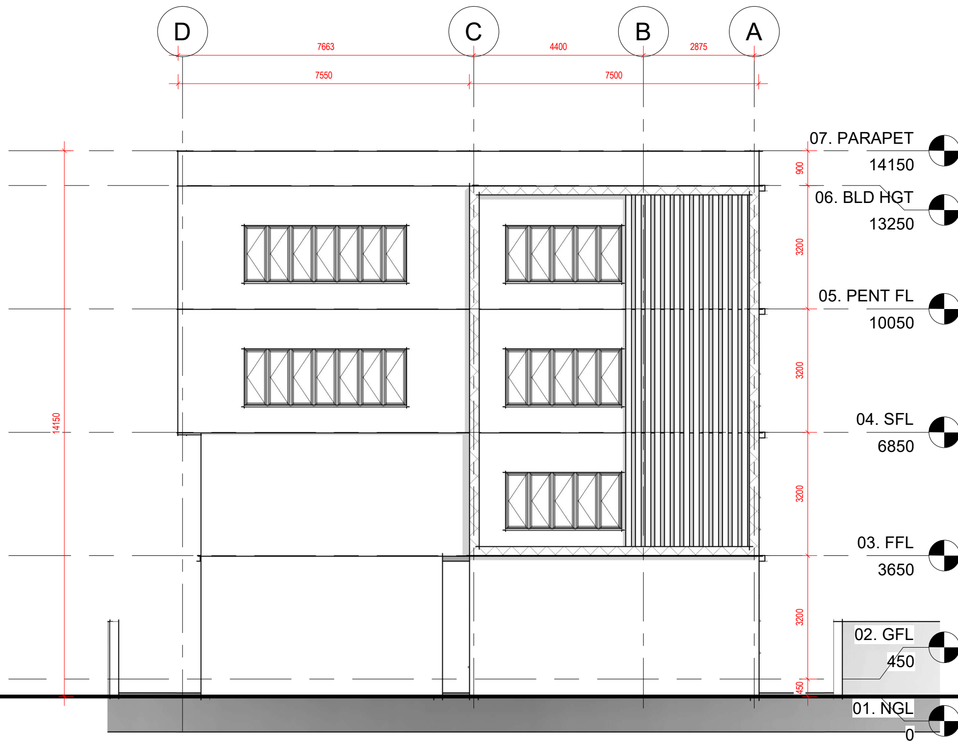
LEFT SIDE VIEW
