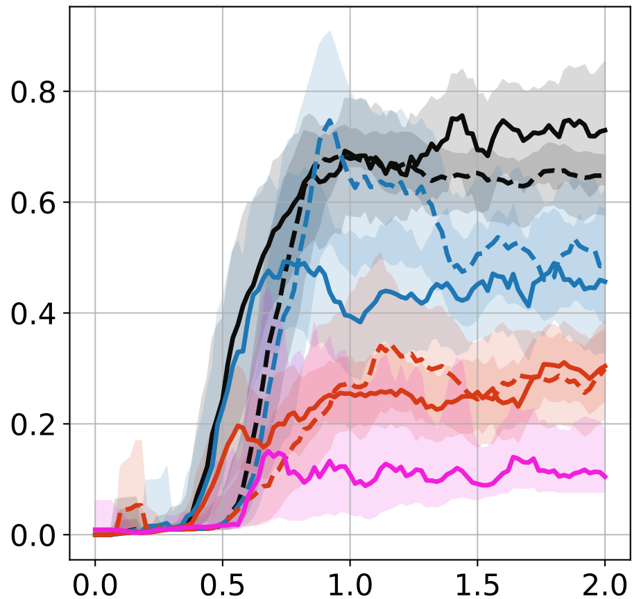
BRIDGE
