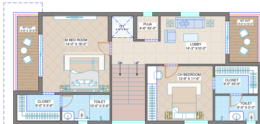
FIRST FLOOR PLAN (1280 SFT) 200 SQYDS WEST
