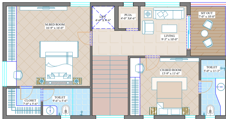
FIRST FLOOR PLAN (1065 SFT) 180 SQYDS EAST
