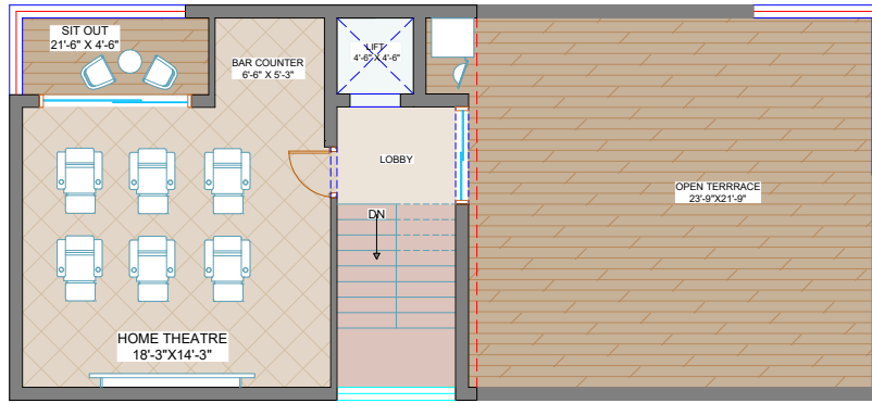
SECOND FLOOR PLAN (620 SFT) 200 SQYDS EAST
