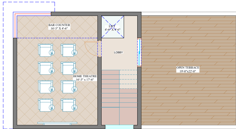
SECOND FLOOR PLAN (640 SFT) 180 SQYDS WEST
