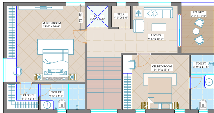
FIRST FLOOR PLAN (1065 SFT) 180 SQYDS WEST
