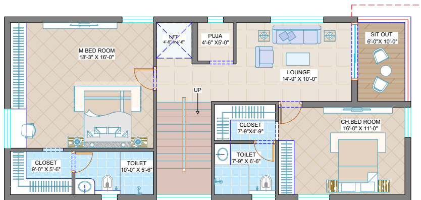
FIRST FLOOR PLAN (1280 SFT) 200 SQYDS EAST
