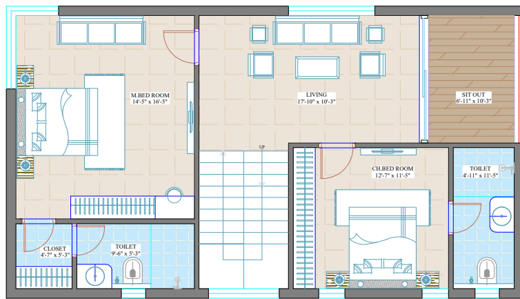
FIRST FLOOR PLAN (980 SFT) 167 SQYDS WEST
