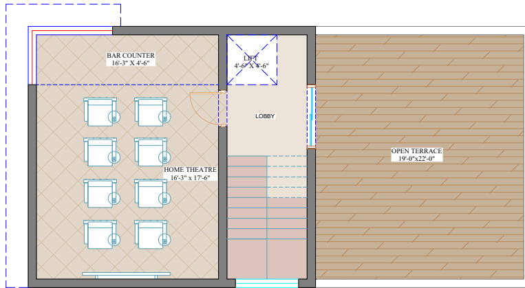
SECOND FLOOR PLAN (640 SFT) 180 SQYDS EAST
