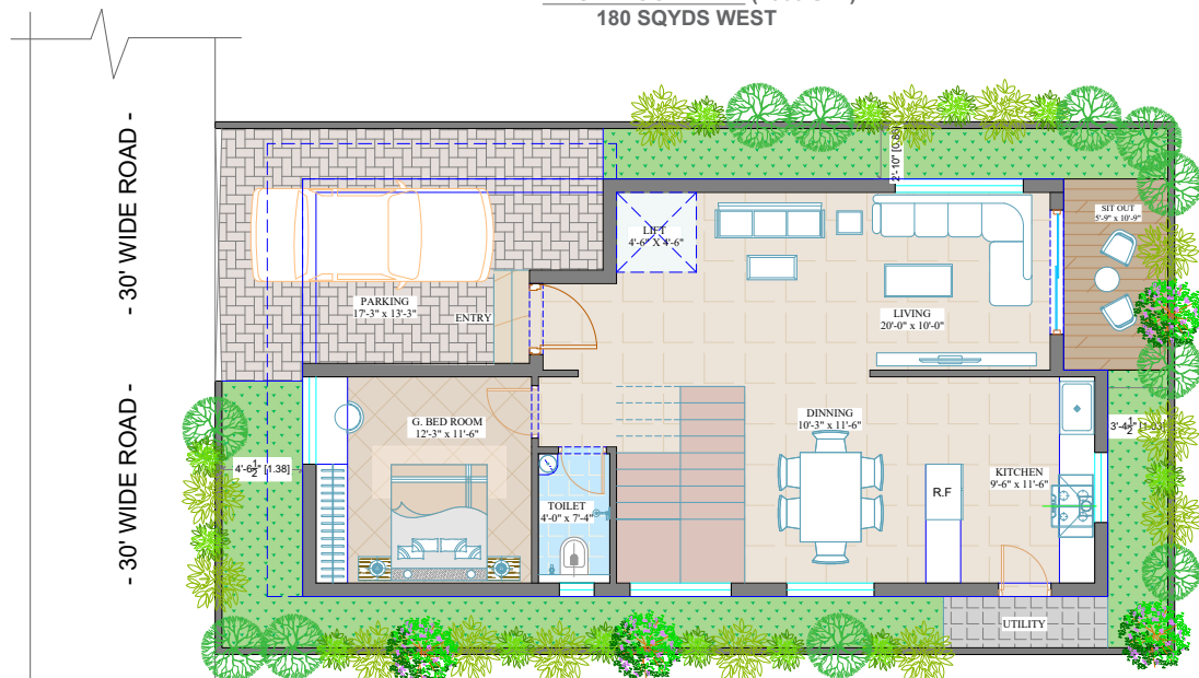
GROUND FLOOR PLAN (1065 SFT) 180 SQYDS WEST
