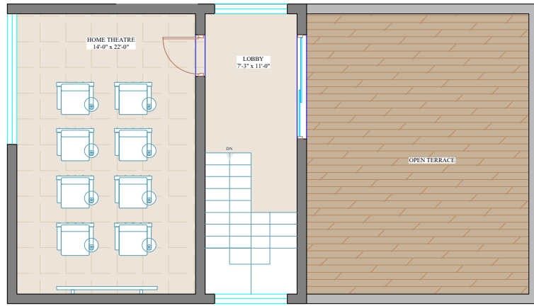
SECOND FLOOR PLAN (540 SFT) 167 SQYDS WEST
