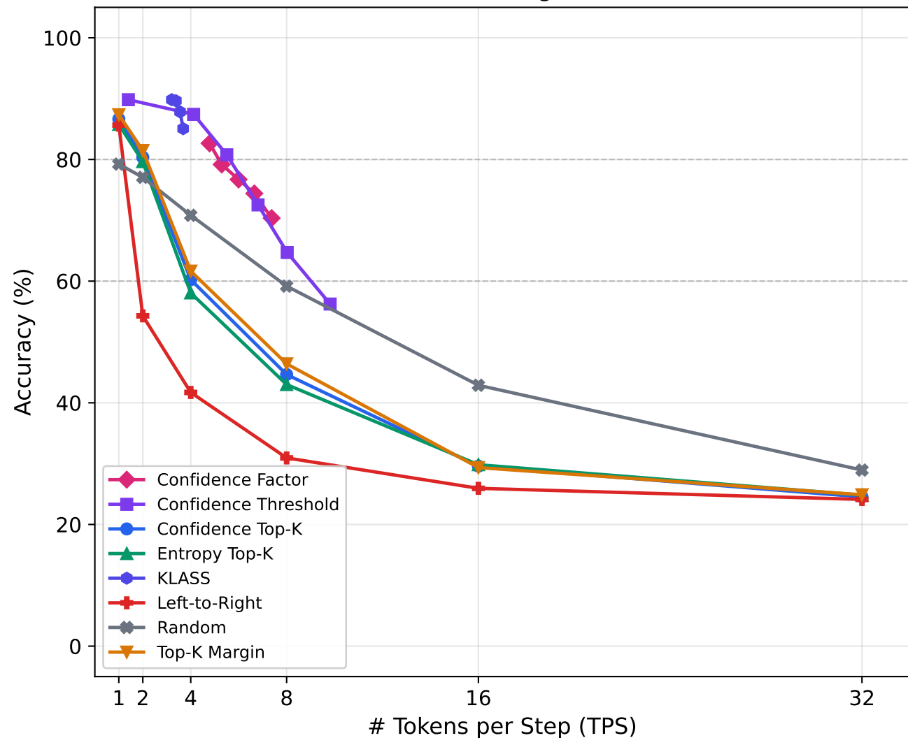
Dream 7B — Average (All Tasks)
