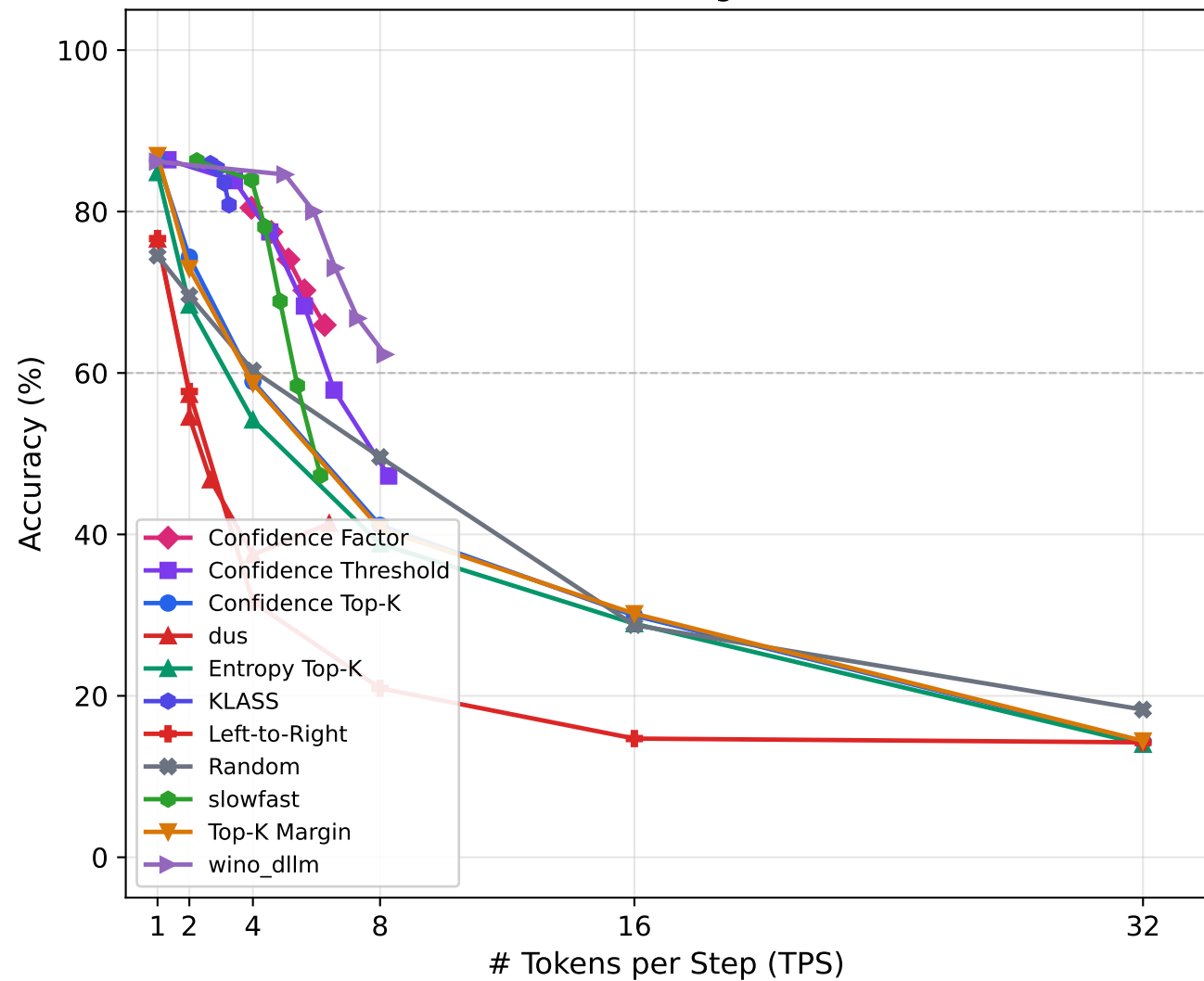
LLaDA 1.5 — Average (All Tasks)
