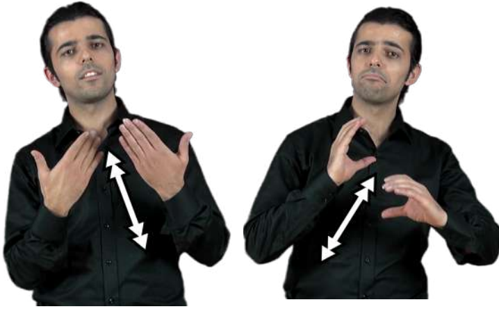
SOHBET (TİD)
