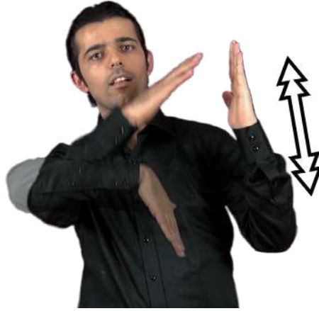
SNFB+
