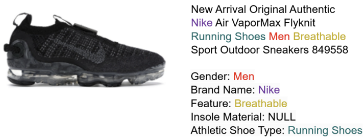
Figure 2.10: Product attribute extraction [38]
