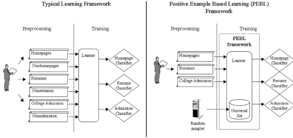
Figure 2.6: Typical framework vs. using PEBL [28]
