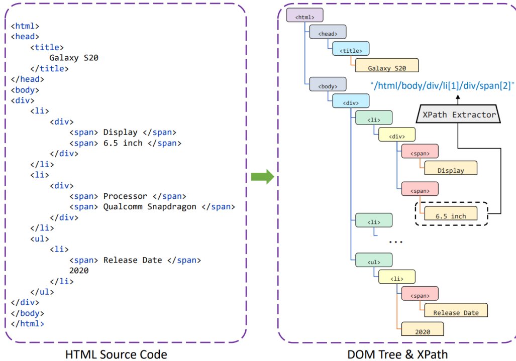
Figure 2.7: DOM tree and XPath in HTML documents [30]
