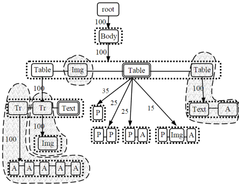
Figure 2.4: An example of site style trees (SST) [17]
