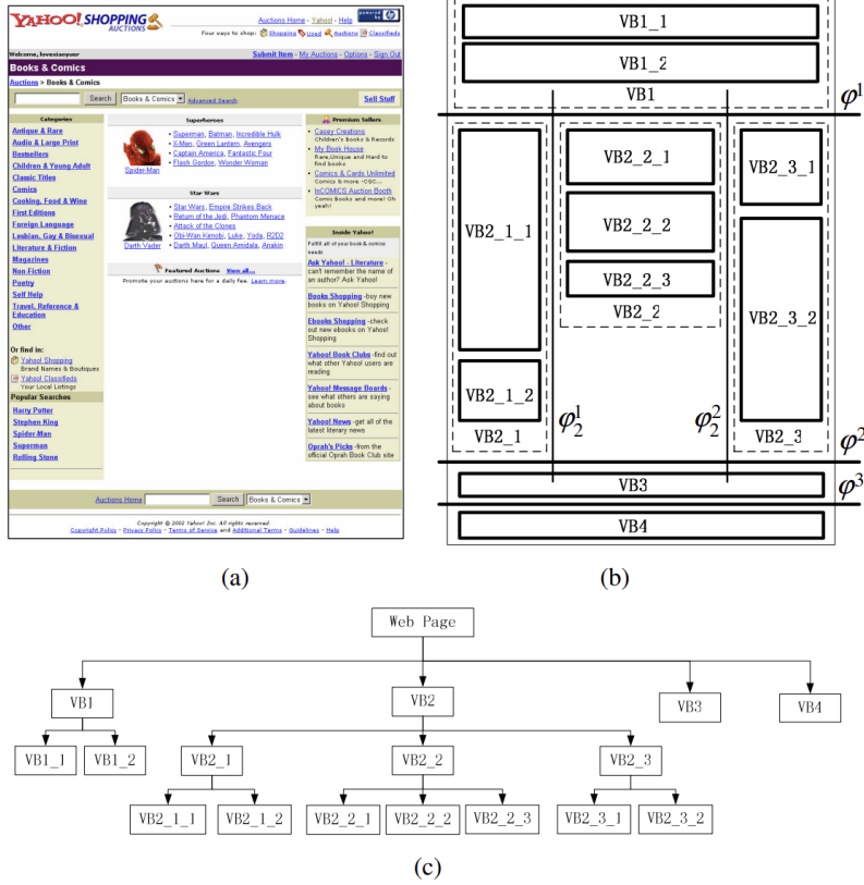
Figure 2.8: Image segmentation of a webpage using the VIPS algorithm [36]
