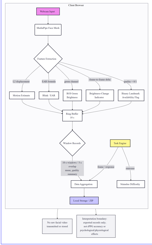
Fig.1 Overview of the Camera System Architecture. The system runs entirely client-side; processing browser obtains webcam frames via MediaPipe Face Mesh (Wasm) to extract rPPG, extracts face-derived exported fields, aggregates 10-s window records, synchronizes them with task events, and Head Motion signals in real-time exports local CSV/ZIP logs. Data is synchronized with Under the Psychophysics Task Engine (Canvas API) and stored locally tested implementation, ensuring no only extracted fields and task events are logged; raw facial video ever leaves the user's device is neither transmitted nor stored by Camera.
