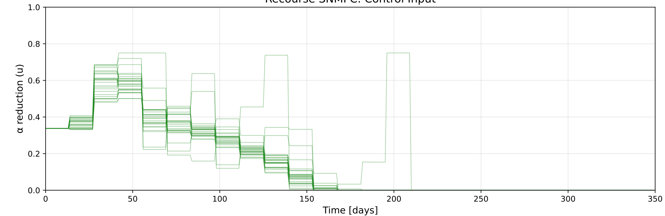
Recourse SNMPC: Control Input
