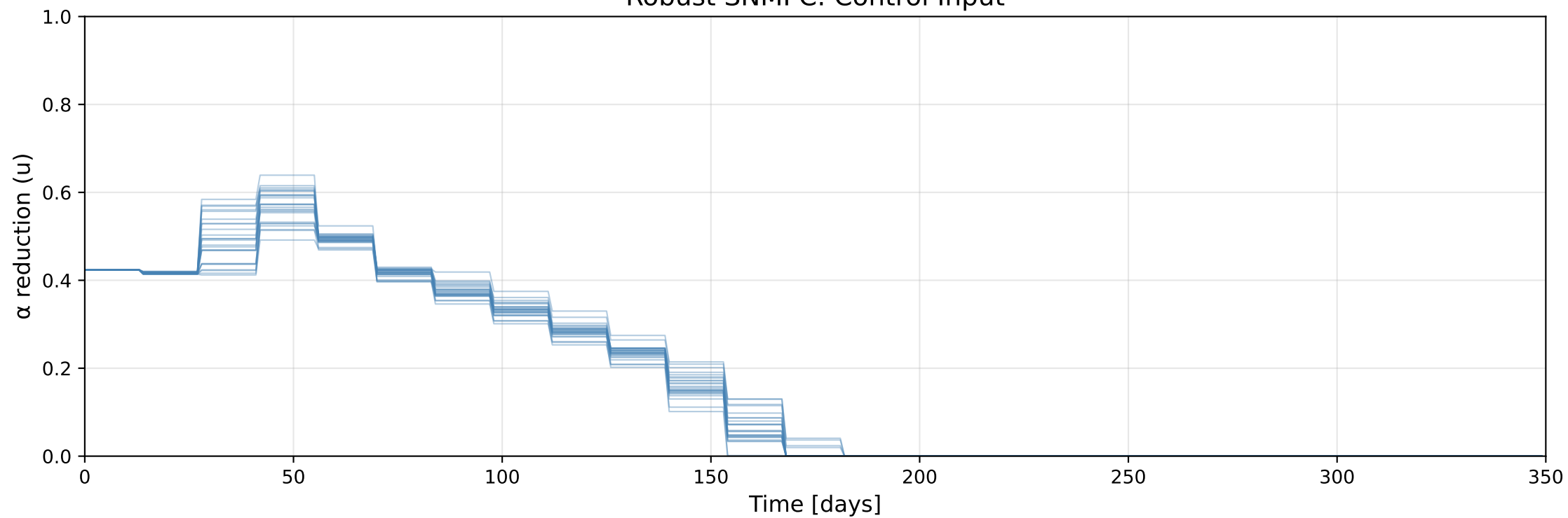
Robust SNMPC: Control Input
