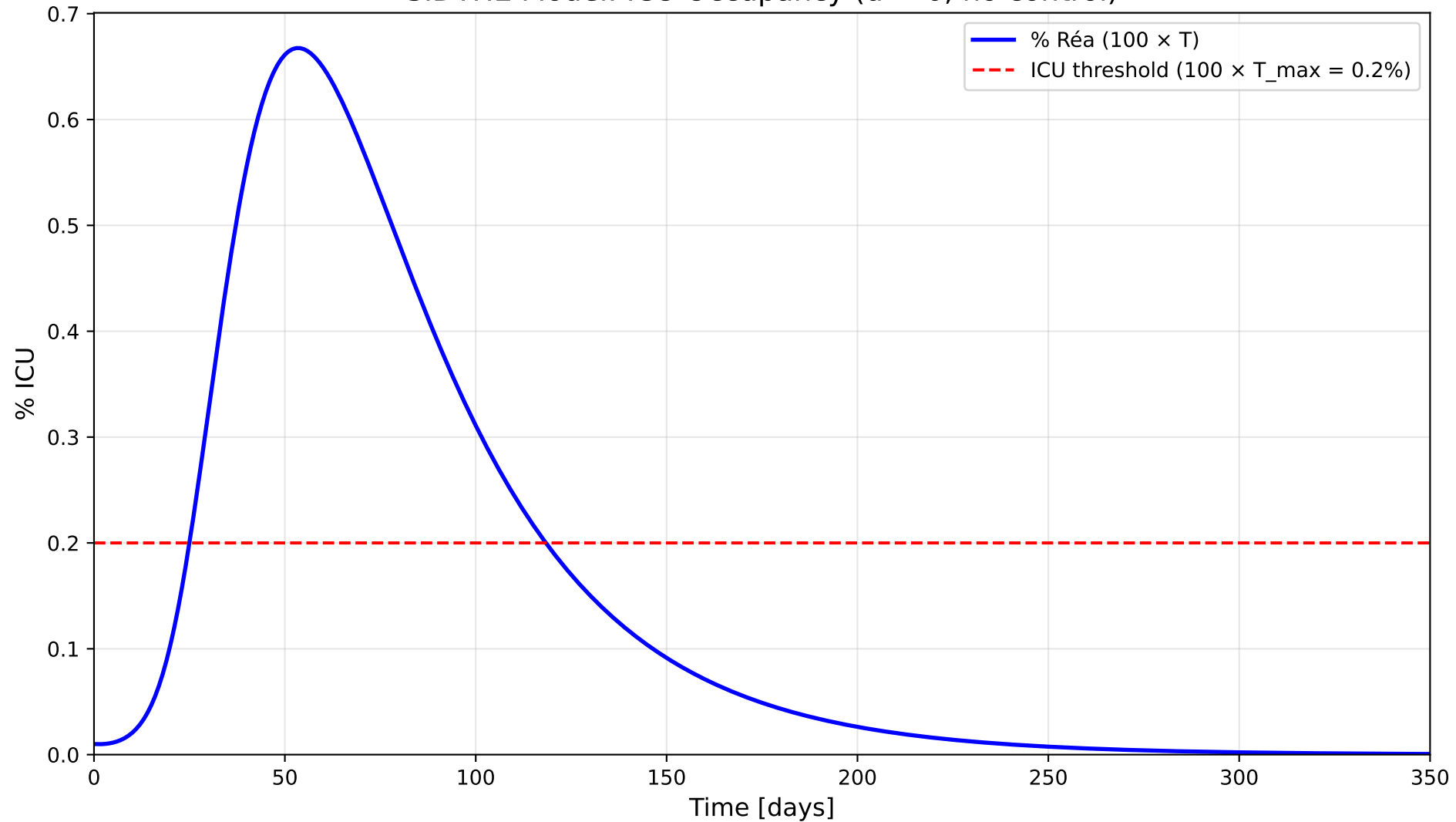
SIDTHE Model: ICU Occupancy ( u = 0 , no control)
