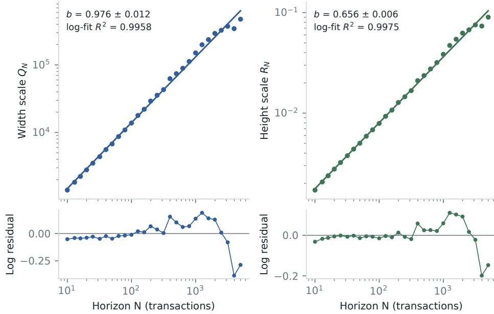
Figure 12. Power-law fits for the estimated width and height scales. Lower panels show log residuals. The displayed R^2 values describe these 28 in-sample points only.
