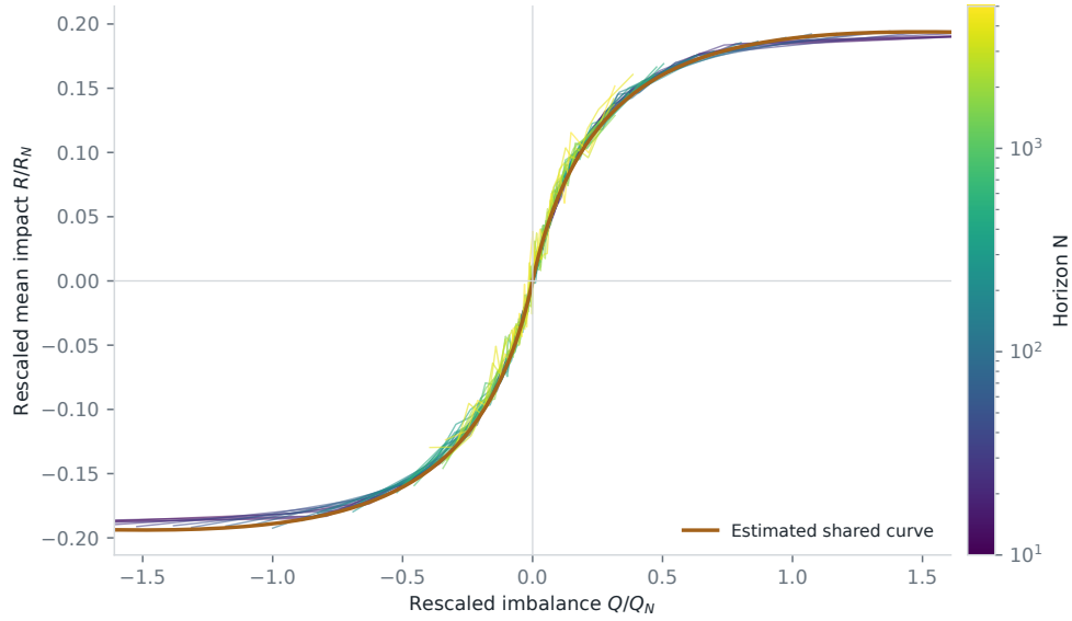
Figure 11. Finite-size scaling collapse for TSLA 2019. Color identifies the aggregation horizon. The orange line is the common fitted shape. This is an in-sample curve construction, not a forecast evaluation.
