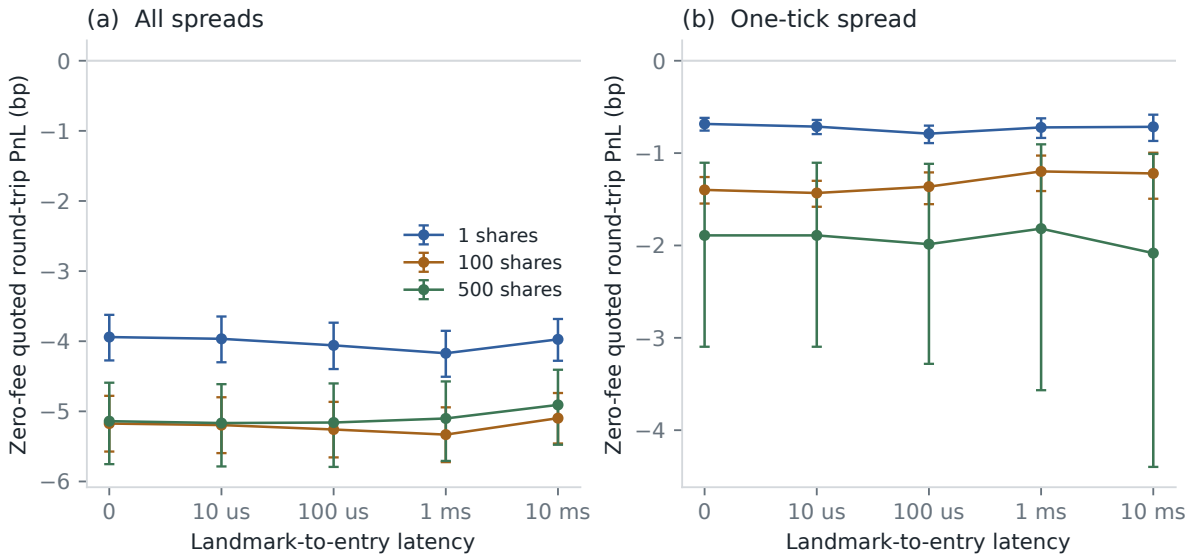
Figure 11. Zero-fee quoted round trips after the fixed price-spell landmark. Both entry and exit walk up to two displayed levels. Bars are complete-date 95 percent intervals; missing tail points have no fully displayed round trip.
