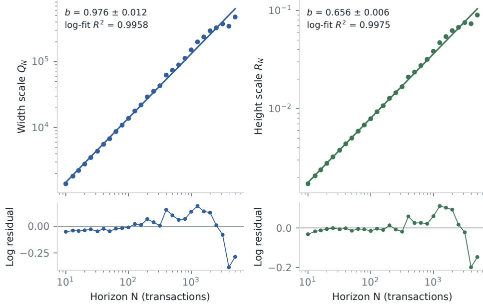
Figure 13. Power-law fits for the estimated width and height scales. Lower panels show log residuals. The displayed R^2 values describe these 28 in-sample points only.
