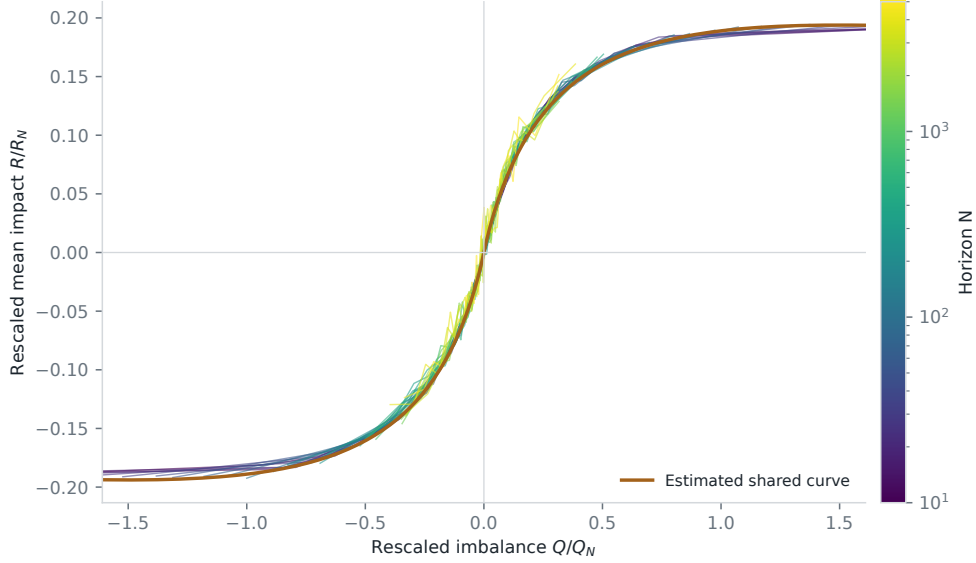
Figure 12. Finite-size scaling collapse for TSLA 2019. Color identifies the aggregation horizon. The orange line is the common fitted shape. This is an in-sample curve construction, not a forecast evaluation.
