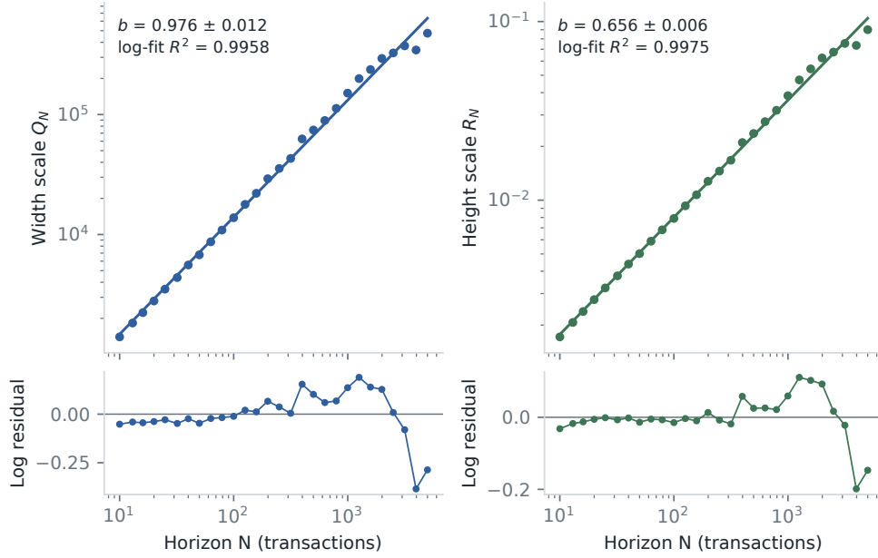
Figure 14. Power-law fits for the estimated width and height scales. Lower panels show log residuals. The displayed R^2 values describe these 28 in-sample points only.
