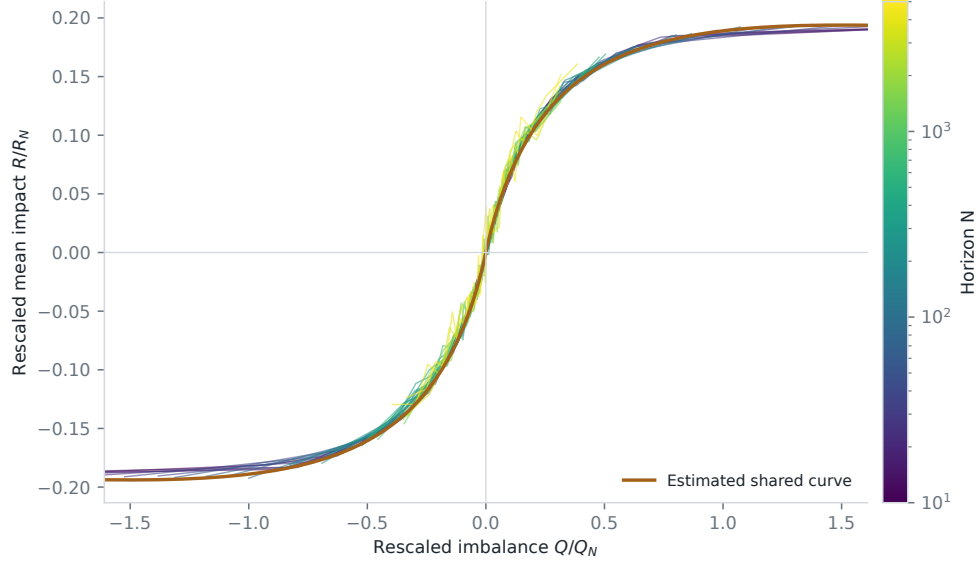
Figure 7. Finite-size scaling collapse for TSLA 2019. Color identifies the aggregation horizon. The orange line is the common fitted shape. This is an in-sample curve construction, not a forecast evaluation.
