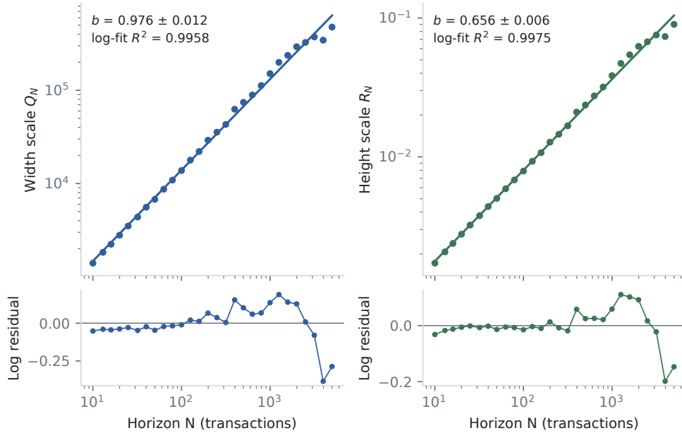
Figure 8. Power-law fits for the estimated width and height scales. Lower panels show log residuals. The displayed R^2 values describe these 28 in-sample points only.
