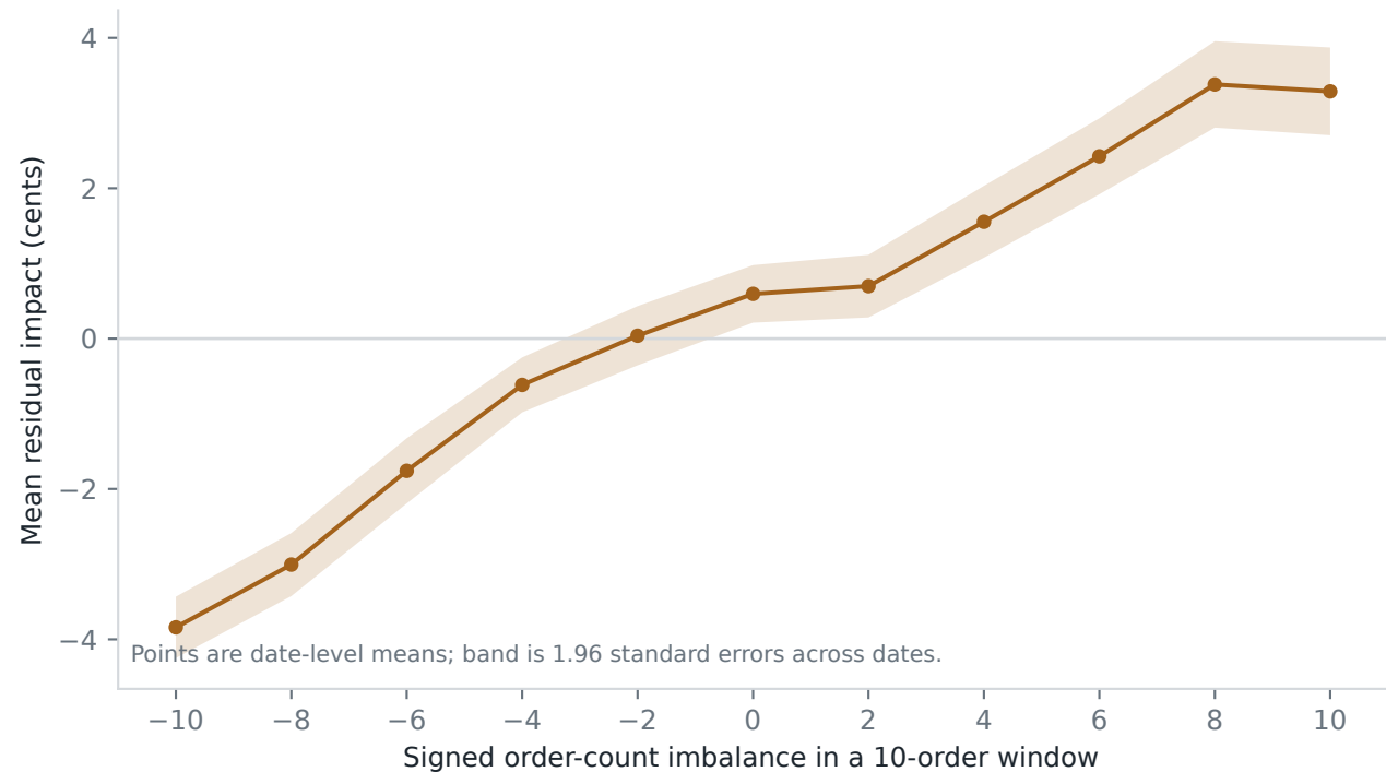
Holdout residual after fitting signed-volume transforms
