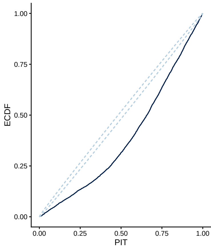
Biased \rightarrow Memory (Miscalibrated)
