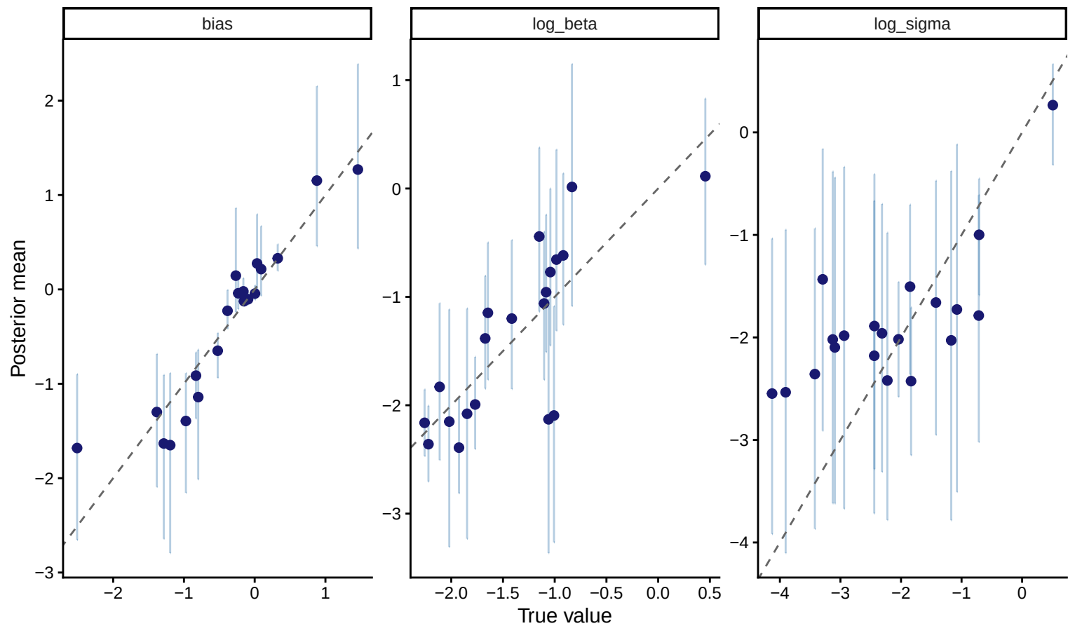
0-ToM parameter recovery (20 synthetic agents, 120 trials)
