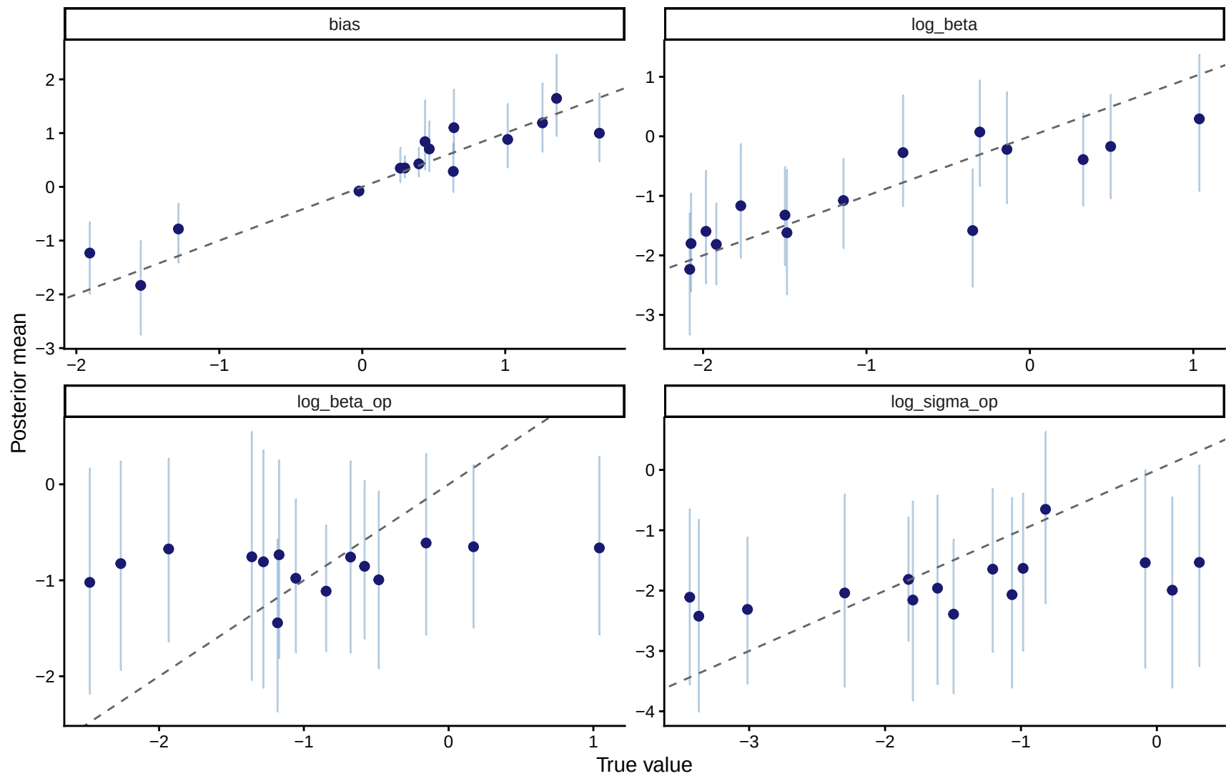
1-ToM parameter recovery (15 synthetic agents, 150 trials)
