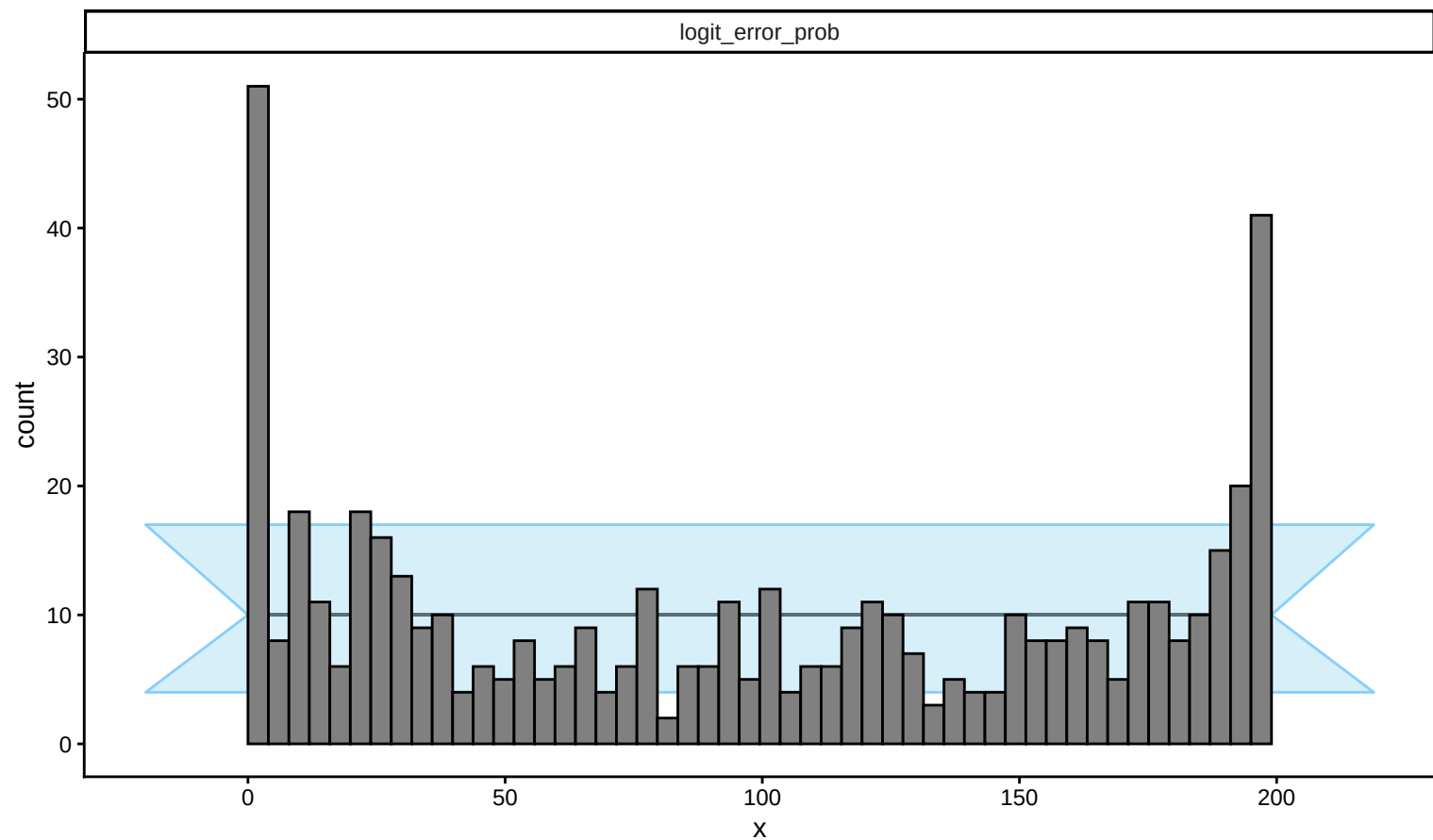
Real SBC rank histogram for Model B
