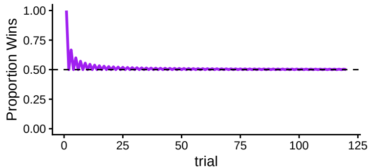
WSLS Performance vs. WSLS
