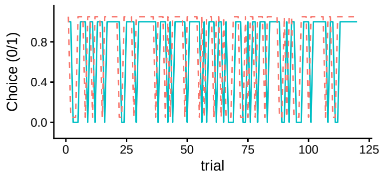
WSLS Performance vs. Biased Random
