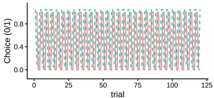
WSLS Performance vs. WSLS
