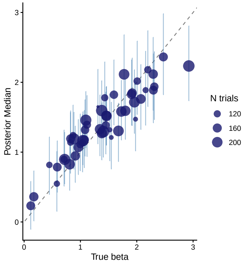
Recovery: Memory Sensitivity \beta_j
