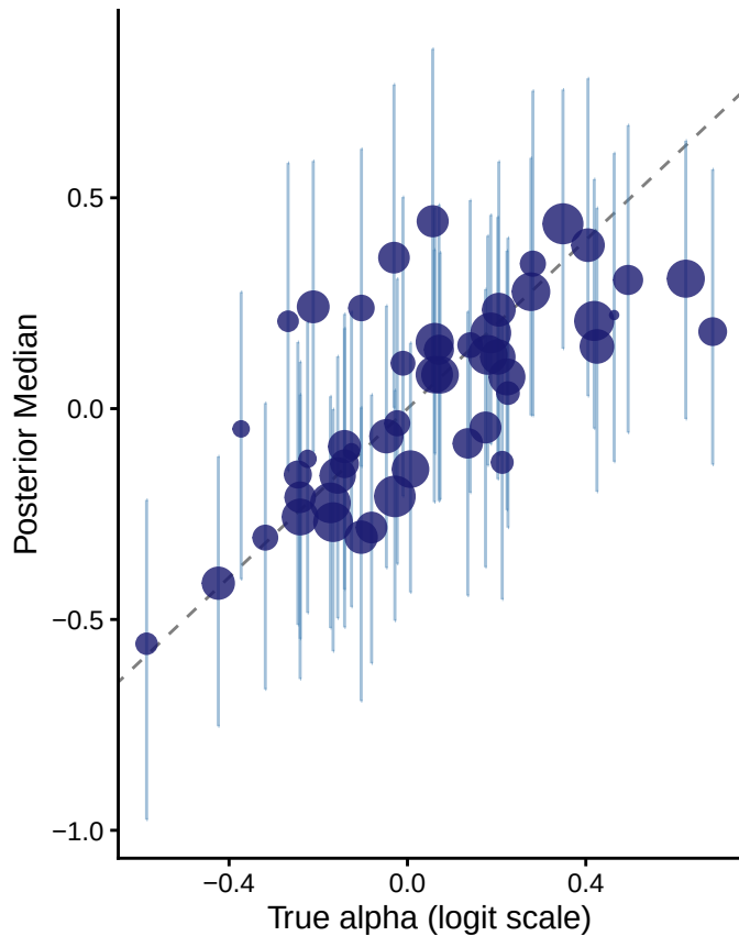
Recovery: Baseline Bias \alpha_j
