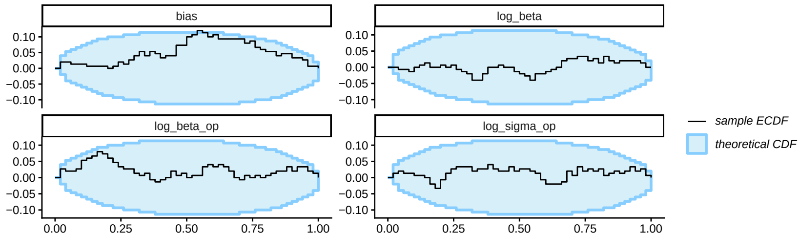
ECDF difference
