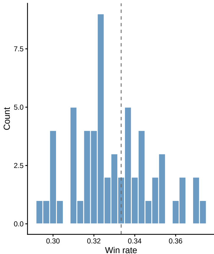
Win rate distribution across players
