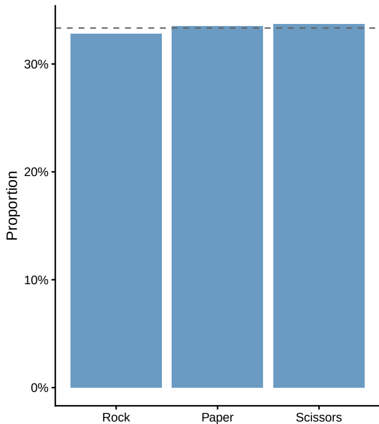
Marginal action distribution
