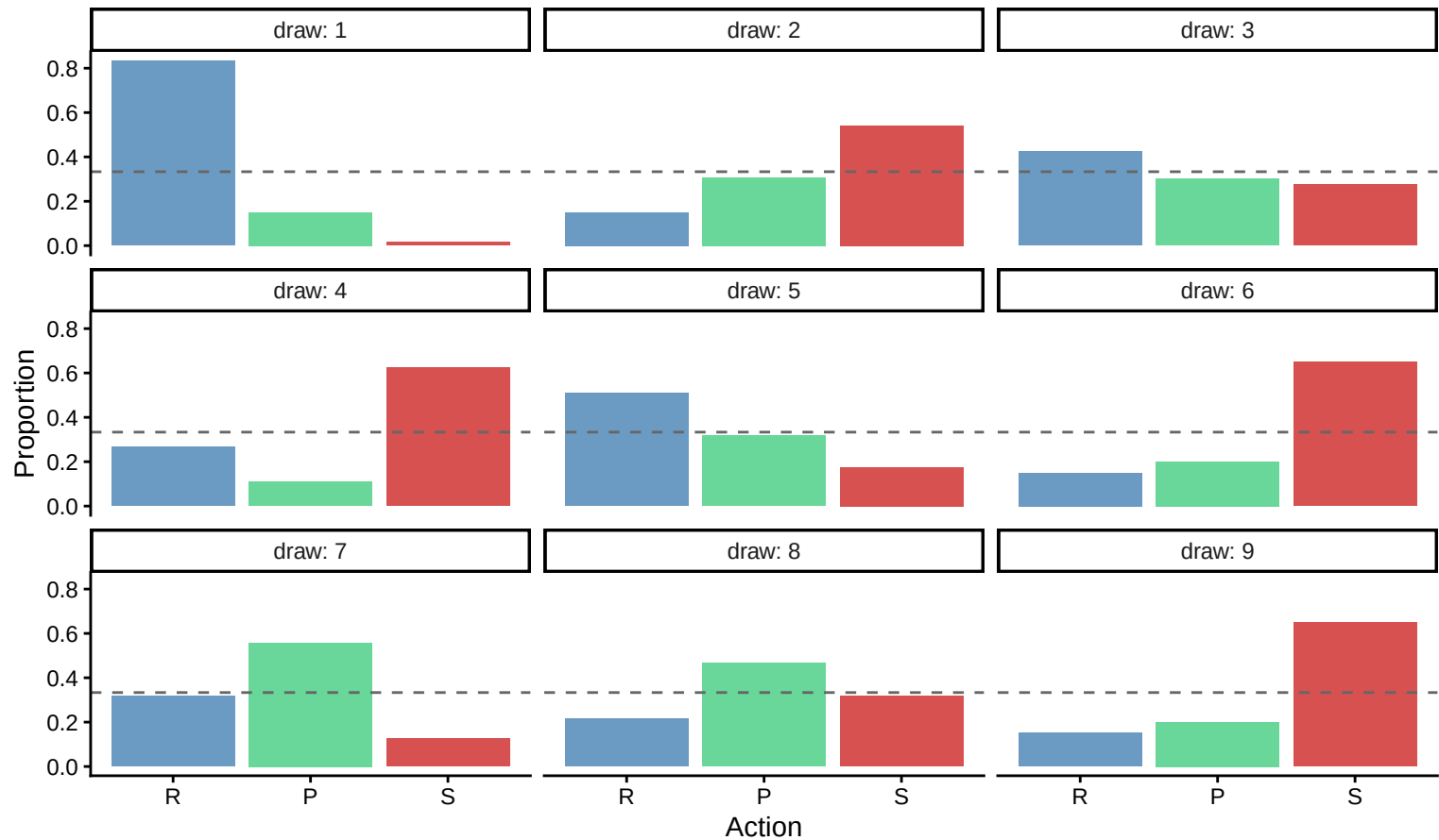
Nash prior predictive: 9 draws from Dirichlet(2,2,2)
