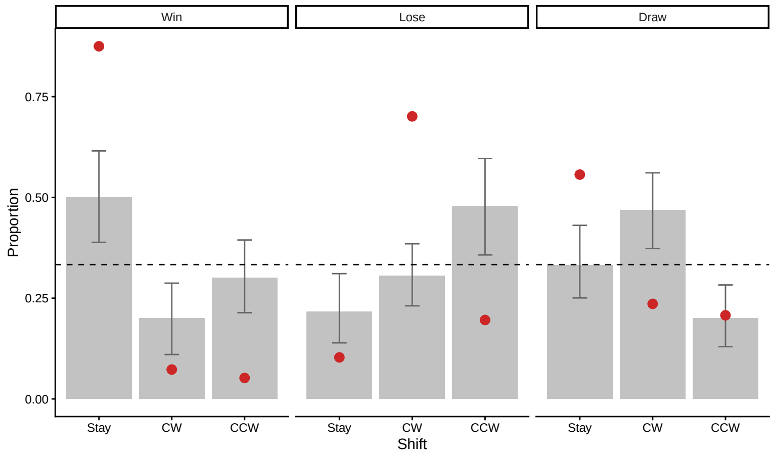
0-ToM posterior predictive vs. observed
